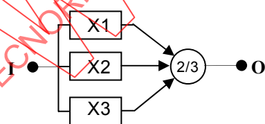
Figure 6 – 2/3 redundancy
