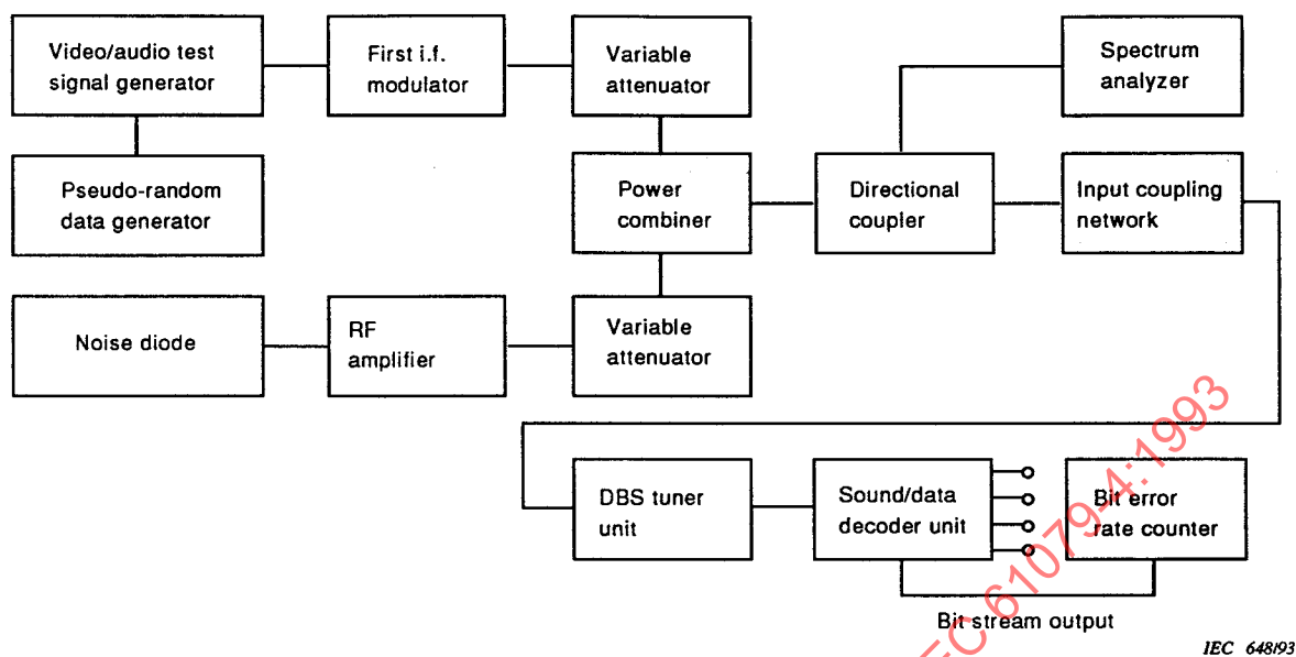
Figure 3 – Arrangement of test equipment for measuring bit error rate
