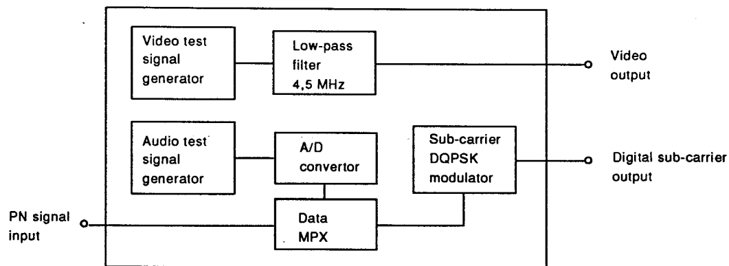
Figure 2a – Video/audio test signal generator
