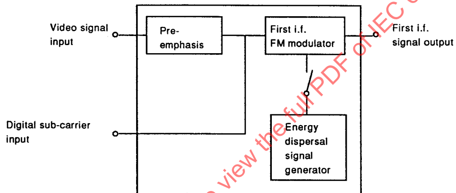
Figure 2b – First i.f. modulator
