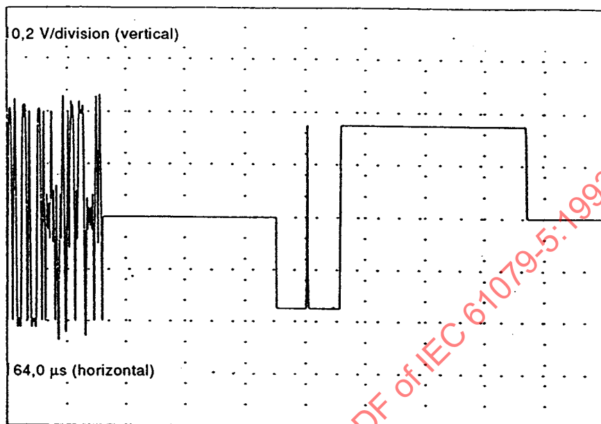
Figure 2e – Pulse and bar luminance signal
