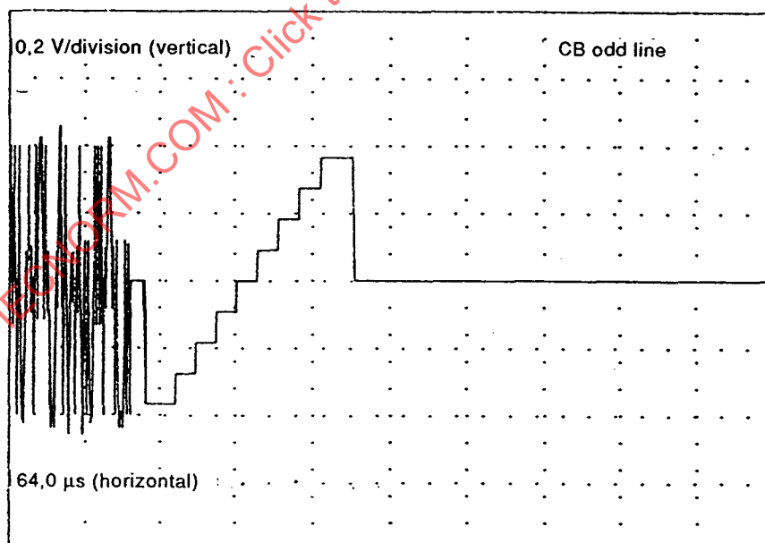
Figure 2g'' – Eight-riser staircase chrominance signal (odd line)
