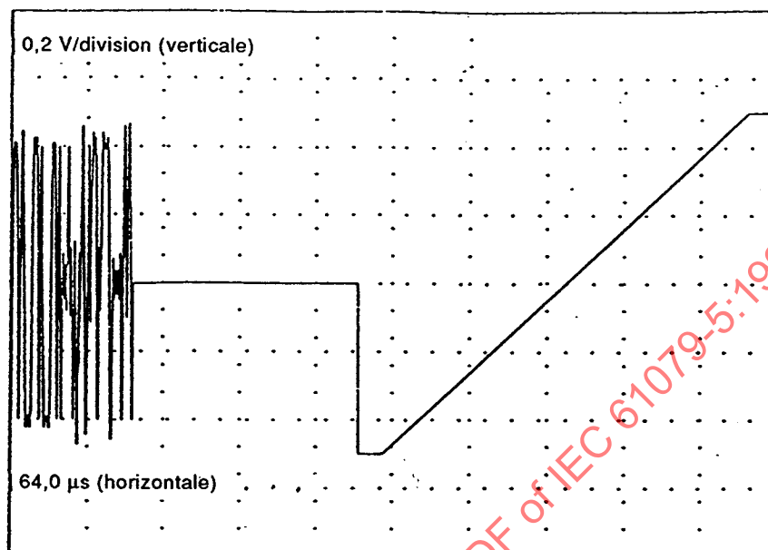
Figure 2f'' – Signal luminance de rampe montante
