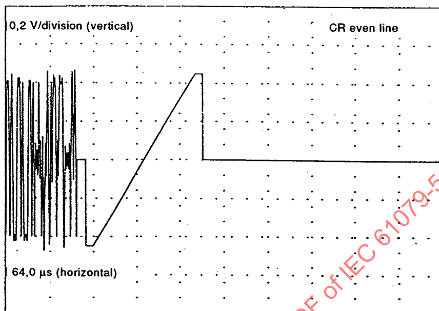
Figure 2f – Rising ramp chrominance signal (even line)
