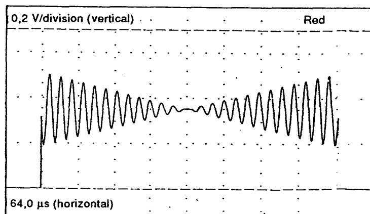
Figure 2j'' – Resulting decoded R colour signal
