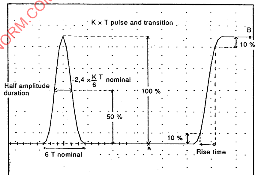
Figure 9 – Pulse response and transition measurements
