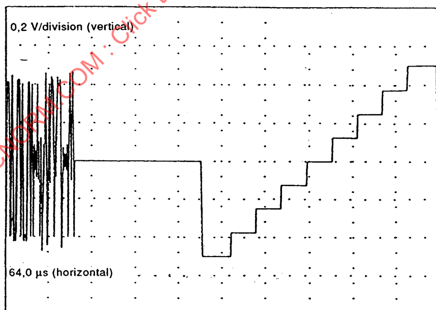
Figure 2g – Eight-riser staircase luminance signal
