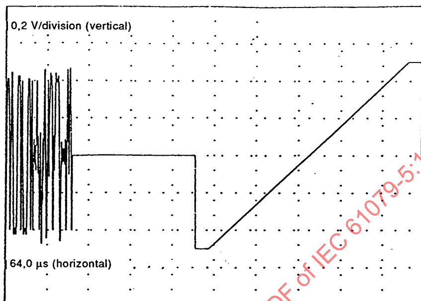
Figure 2f'' – Rising ramp luminance signal
