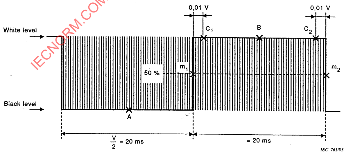
Figure 11 – Low-frequency distortions measurement
