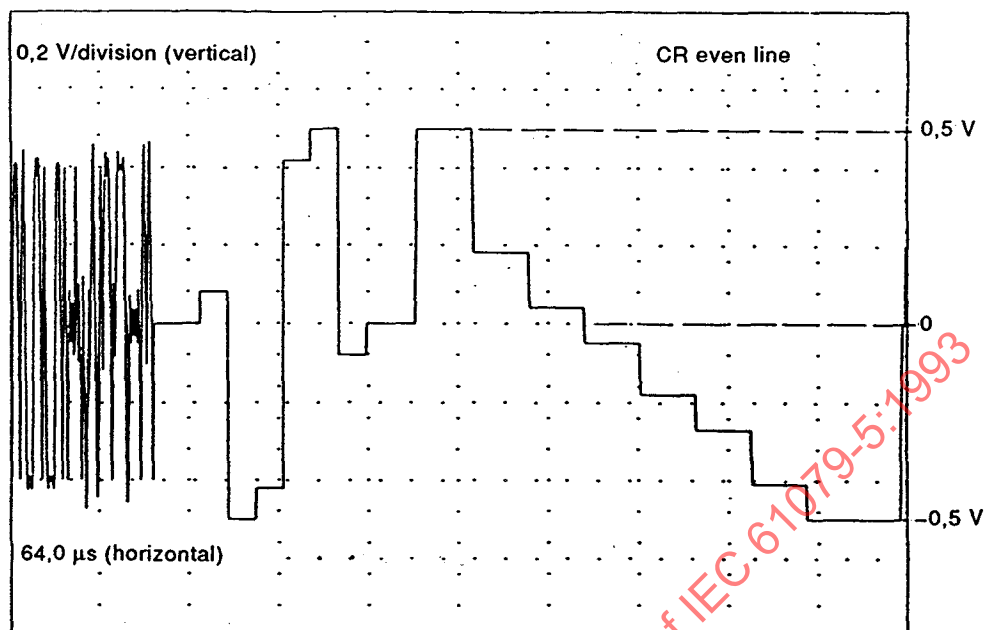
Figure 2i – 75 % colour-bar signals (even line)
