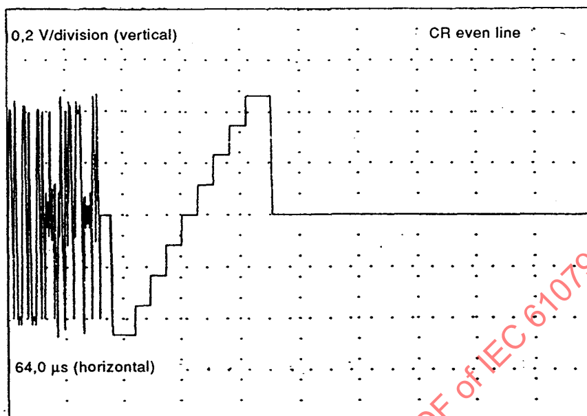
Figure 2g' – Eight-riser staircase chrominance signal (even line)
