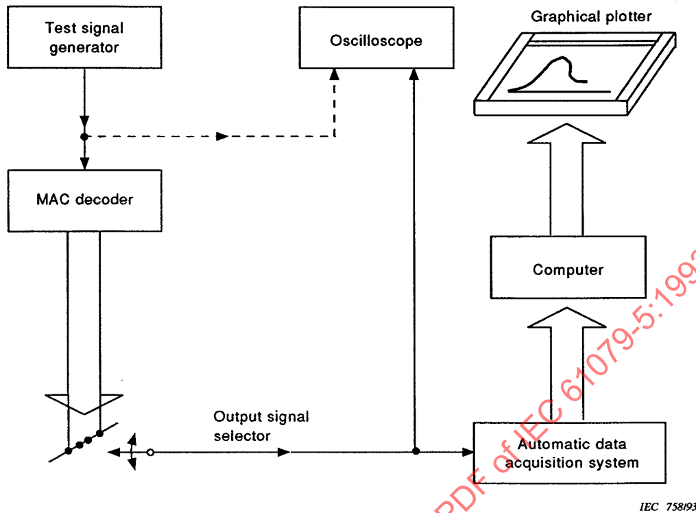
Figure 8 – Circuit arrangement for automatic measurement acquisition and processing
