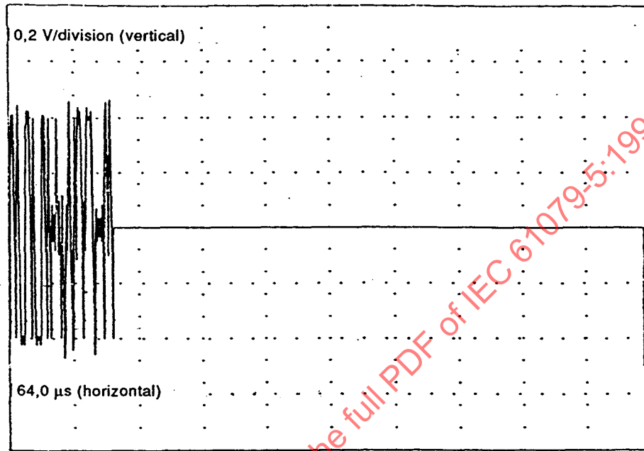
Figure 2h - 50 % grey-level signal
