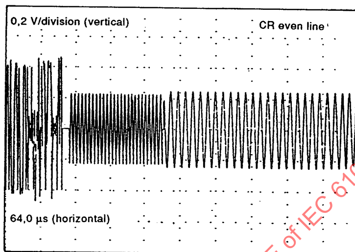
Figure 2j – Bow-tie test signal (even line)
