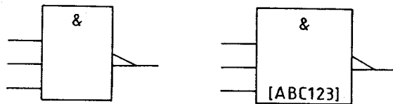
Figure 50 - Example of the use of different symbol sizes; an AND-gate with negated output, without and with additional information.
