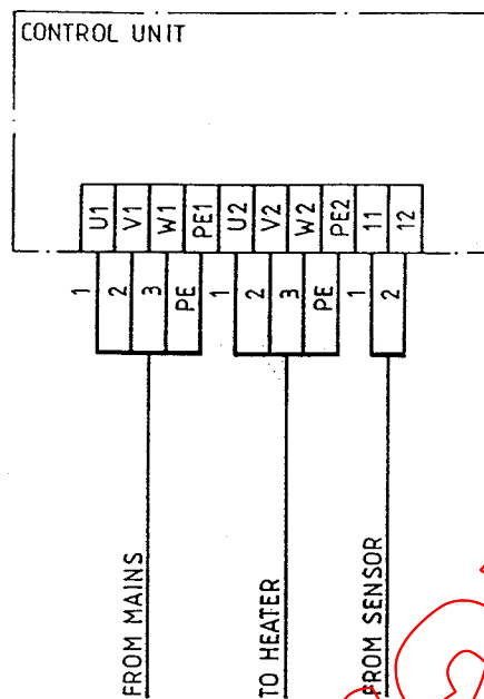
Figure 31 - Example of a terminal connection diagram; a control unit.
