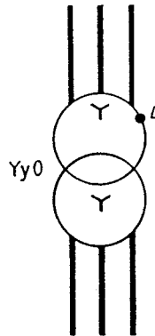
Figure 47 - Example of a symbol supplemented with qualifying symbols for connection of windings and a vector group code; same transformer as in figure 46.
