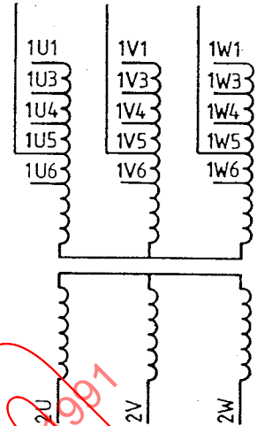
Figure 48 - Example of detailed symbol; same transformer as in figure 46.
