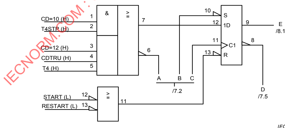
Figure 43 – Detail of a circuit diagram using direct logic polarity convention
