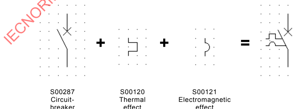
Figure A.6 – Miniature circuit-breaker shown with the symbol for a circuit-breaker qualified with the symbol for thermal and electromagnetic effects
