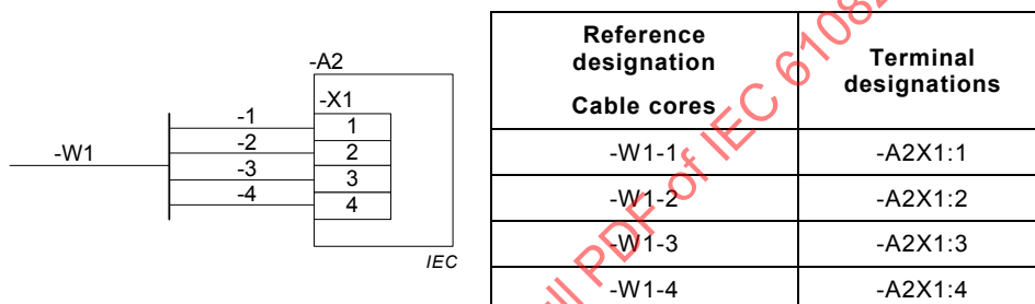
Figure 82 – Example of presentation of termination of a multi-core cable
