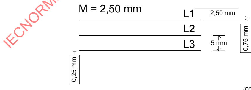
Figure 37 – Spacing of lines
