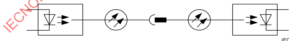
Figure 10 – Example of the use of symbols for fibre optics
