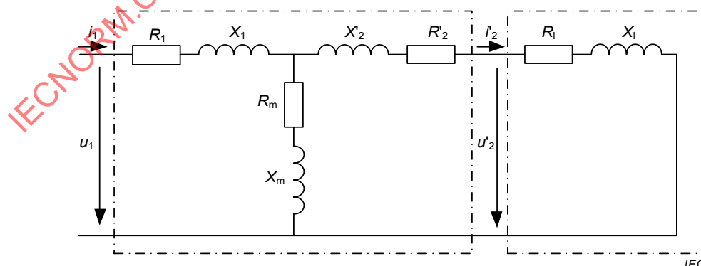
Figure 62 – Example of an equivalent-circuit diagram
