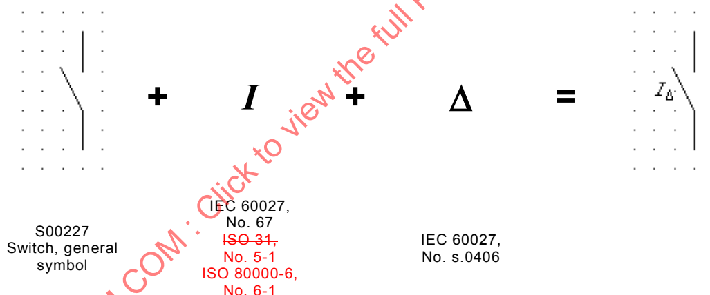
Figure A.10 – Example of a symbol for an RCD
