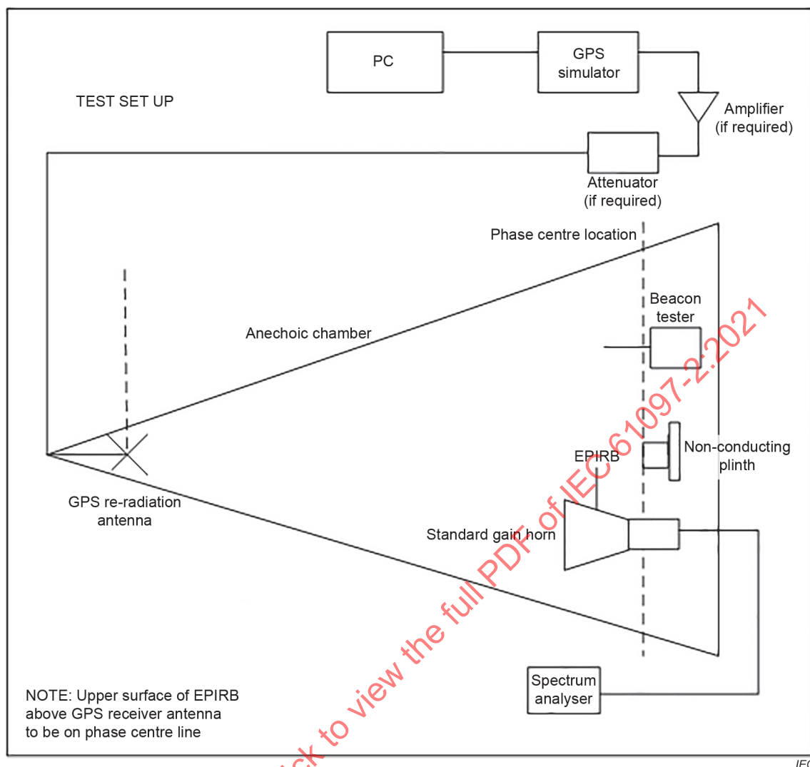
Figure B.1 – Test set-up
