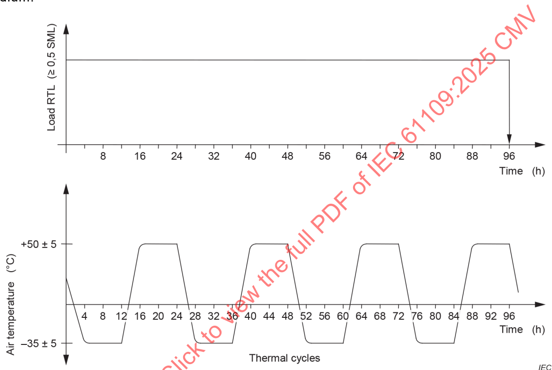
Figure 1 – Thermal-mechanical pre-stressing
