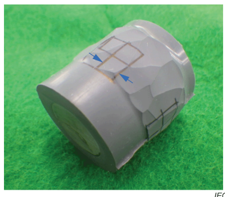
Figure F.5 – Example of test specimen for peel test
