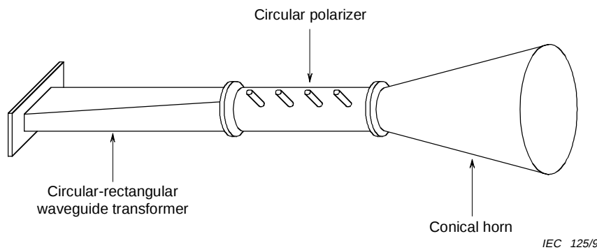
Figure A.1 – Circularly polarized standard antenna
