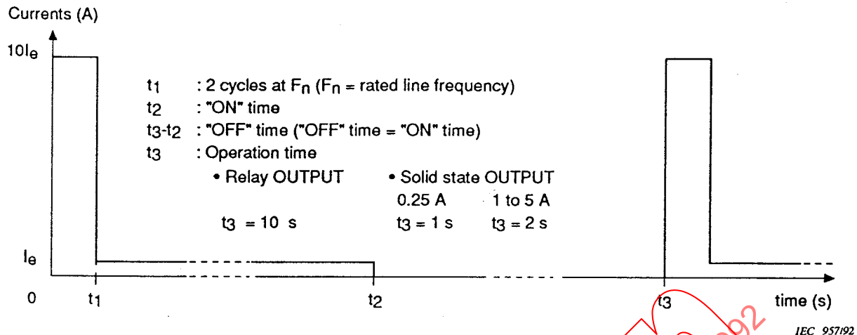
Figure 4 – Temporary overload waveform for digital a.c. outputs
