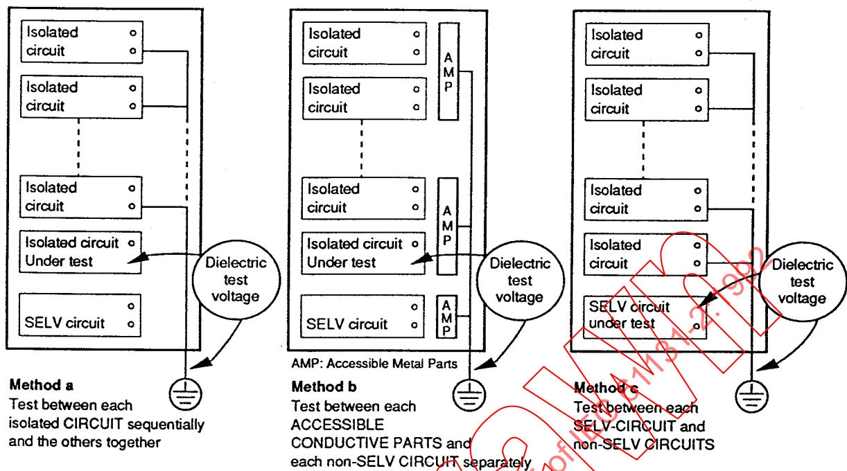
Figure 8 – Dielectric test procedures
