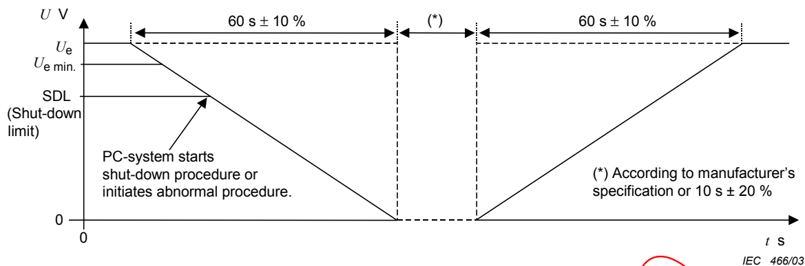
Figure 7 – Gradual shut-down/start-up test
