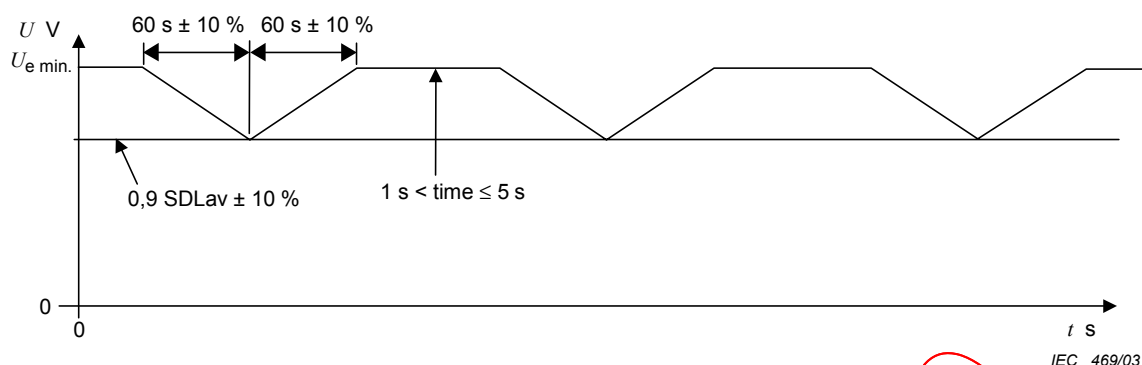
Figure 10 – Slow supply voltage variation test
