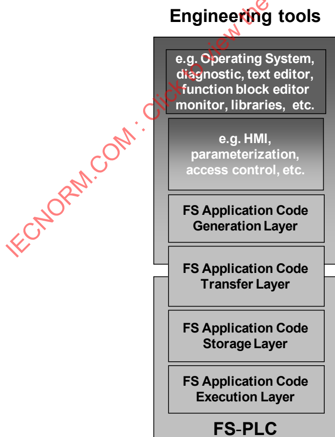
Figure 11 – Model of FS-PLC and engineering tools layers
