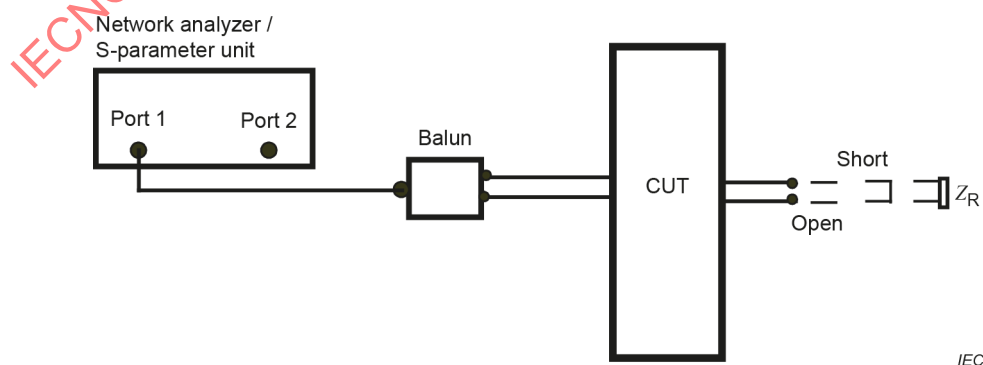
Figure 12 – Test set-up for characteristic impedance, terminated input impedance, and return loss
