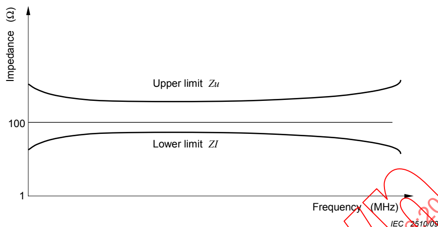
Figure 1 – Impedance template
