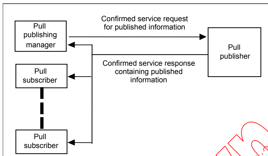
Figure 13 – Pull model interactions
