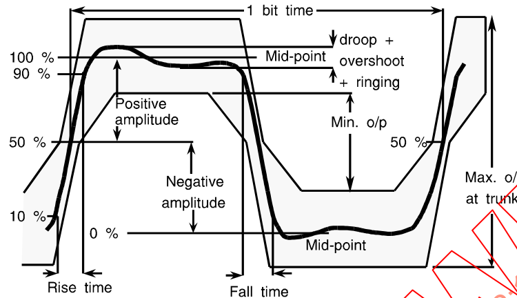
Figure 42 – Output waveform
