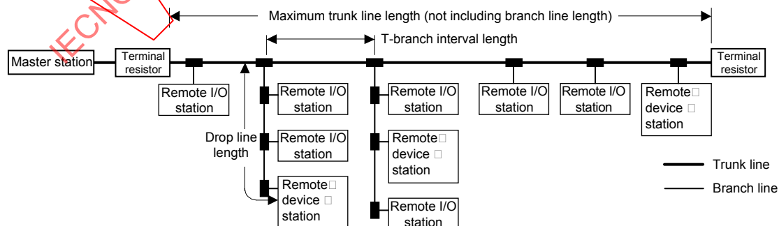
Figure 144 – T-branch topology
