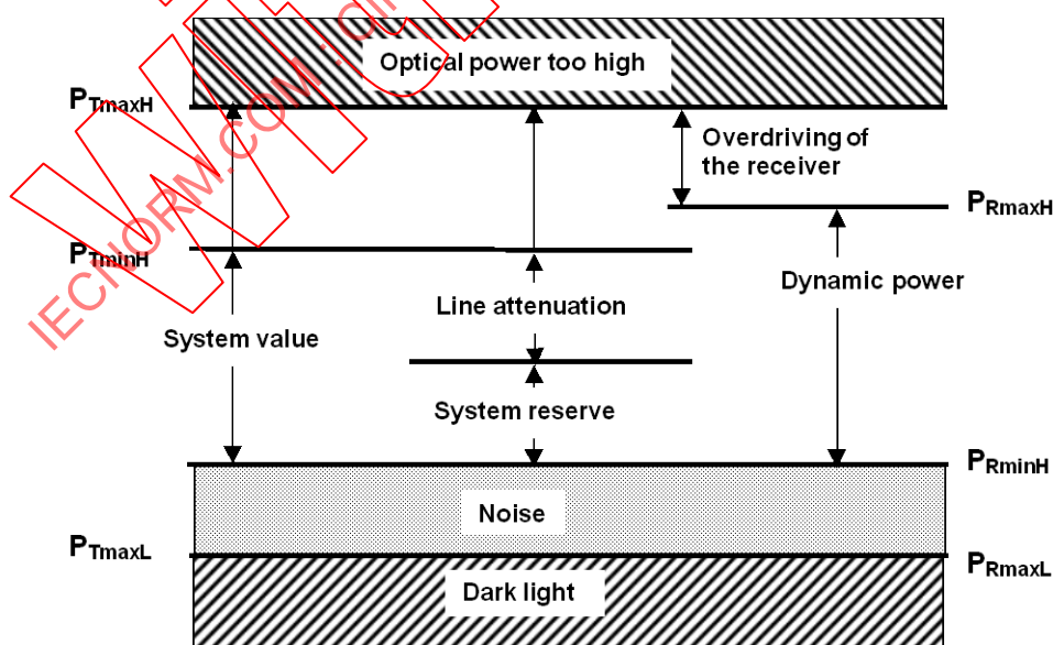
Figure O.3 – Optical power levels
