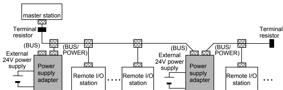
Figure 145 – Type 18-PhL-P power distribution
