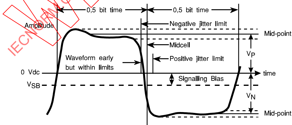
Figure 69 – Transmitted and received bit cell jitter (zero crossing point deviation)
