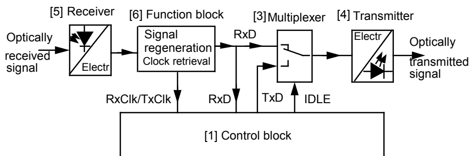
Figure 134 – Functions of a slave connection
