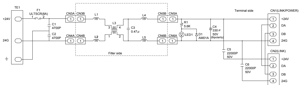
Figure 150 – PhL-P power supply circuit
