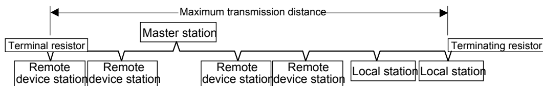
Figure 137 – Dedicated cable topology
