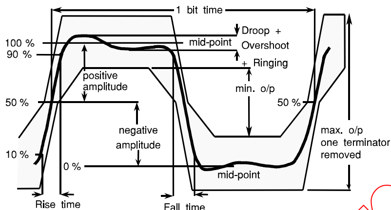
Figure 55 – Output waveform
