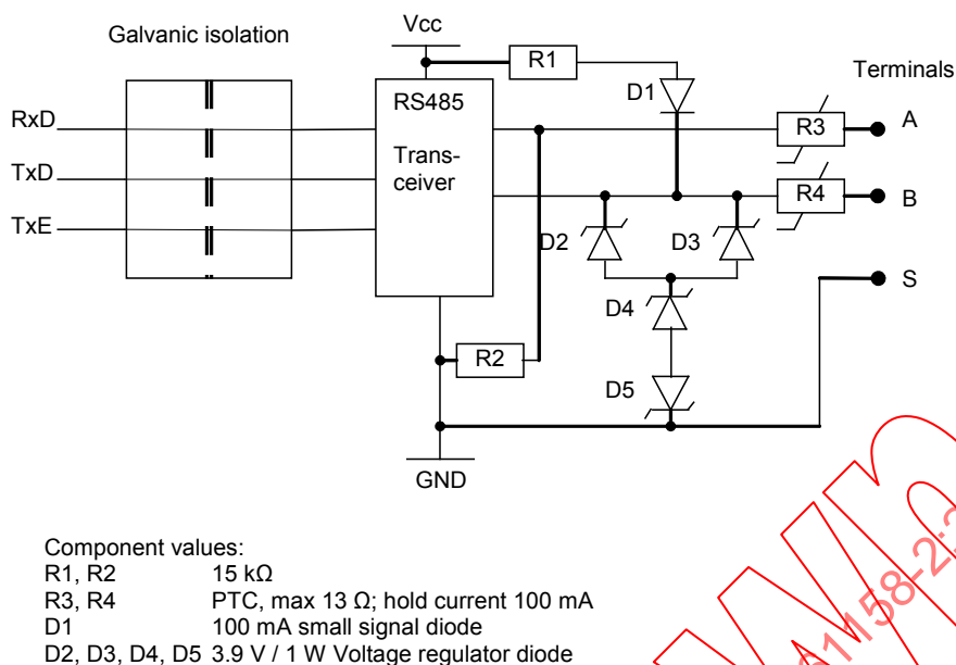
Figure 117 – Recommended interface circuit
