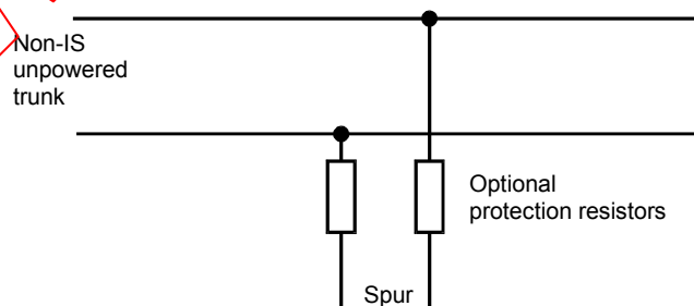
Figure 67 – Protection resistors
