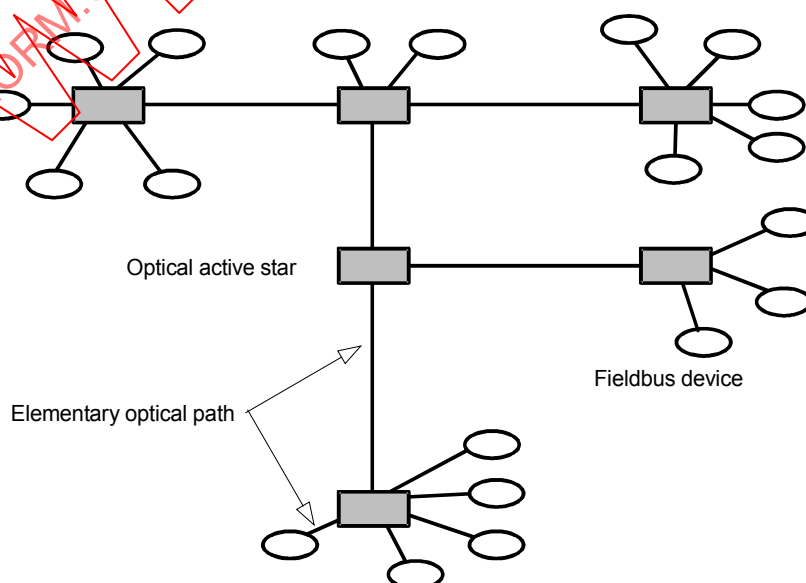
Figure D.2 – Multi-star topology with an optical MAU
