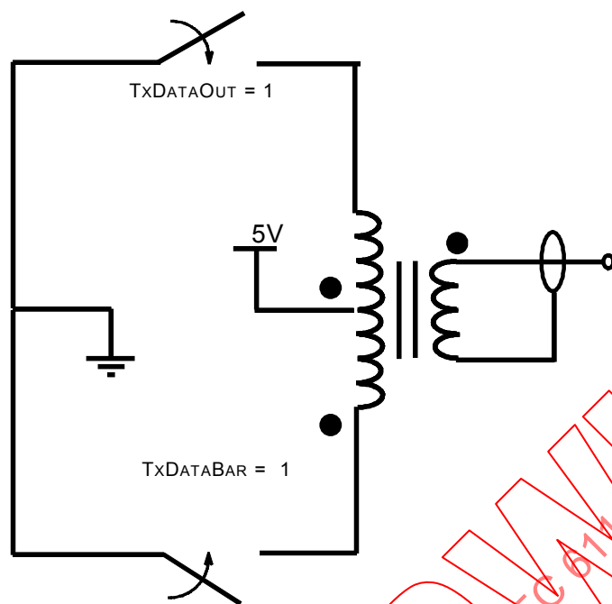
Figure 79 – Coaxial wire MAU transmitter
