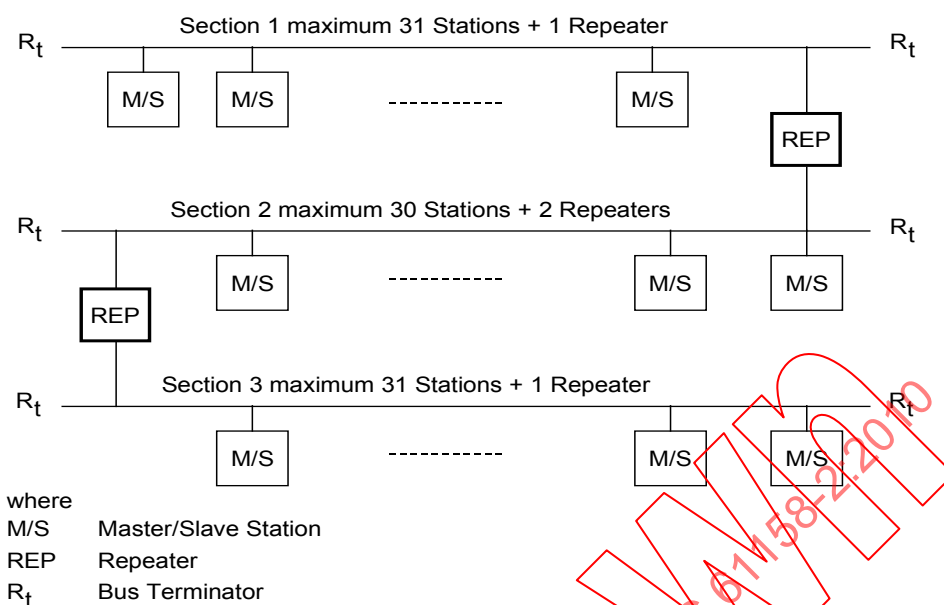
Figure 98 – Repeater in linear bus topology
