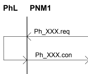
Figure 14 – Reset, Set-value, Get-value PhL services
