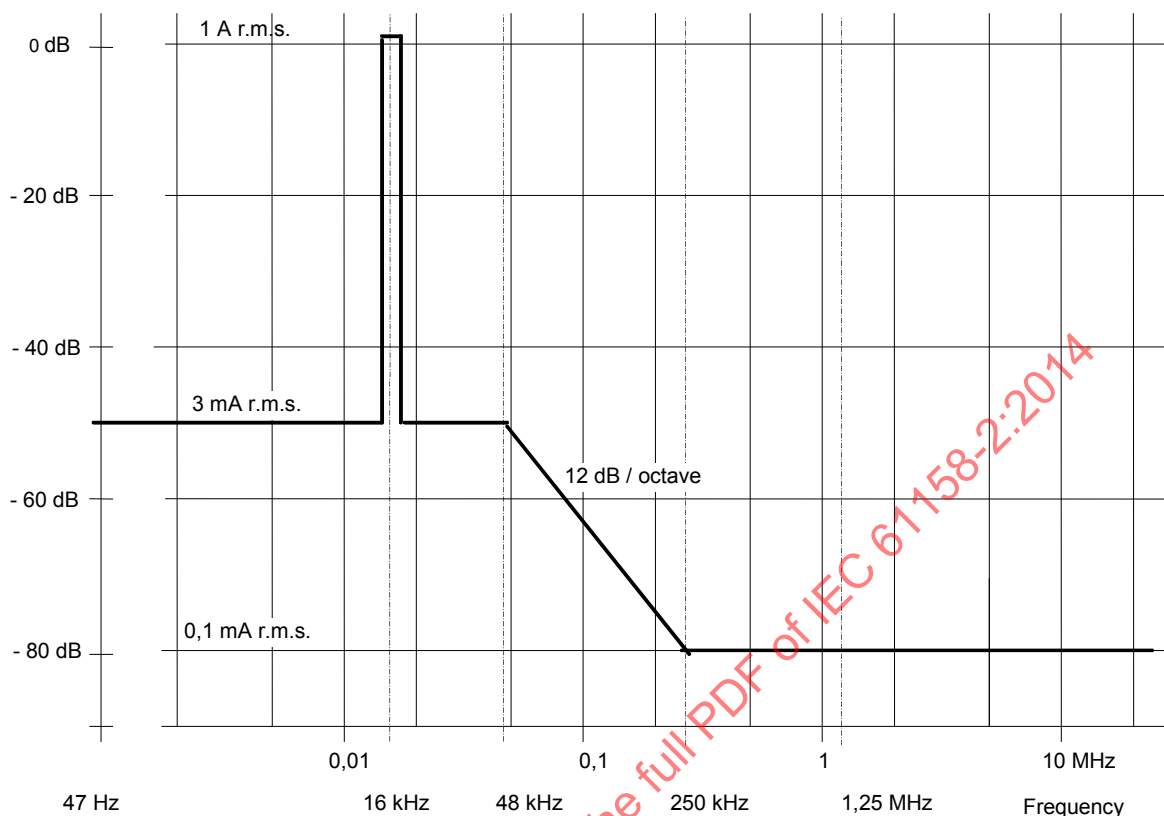
Figure 74 – Power supply harmonic distortion and noise
