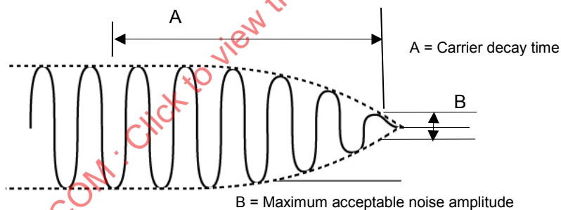
Figure 165 – Carrier decay time
