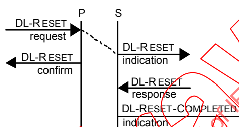
Figure 51 – Sequence of primitives in a publishing DLS-user initiated Reset
