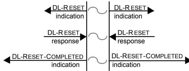
Figure 55 – Sequence of primitives in a peer DLS-provider initiated Reset
