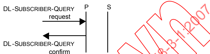
Figure 61 – Sequence of primitives for Subscriber Query
