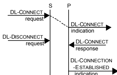
Figure 41 – Sequence of primitives in a DLS-user cancellation of a DLC/DLCEP establishment attempt: subscriber's DL-DISCONNECT request arrives after DL-CONNECT request has been communicated to the publisher
