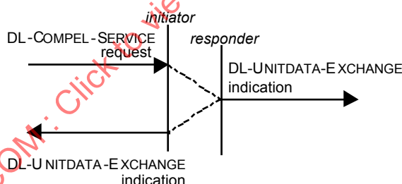
Figure 68 — Sequence of primitives for connectionless-mode unitdata exchange
