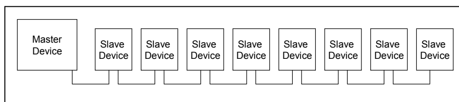
Figure 4 – Type 12 segment in direct mode
