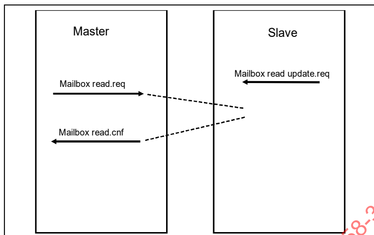
Figure 10 – Successful mailbox read sequence
