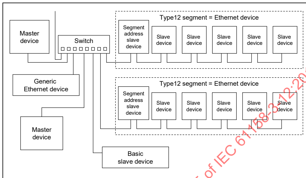
Figure 3 – Type 12 segments in open mode
