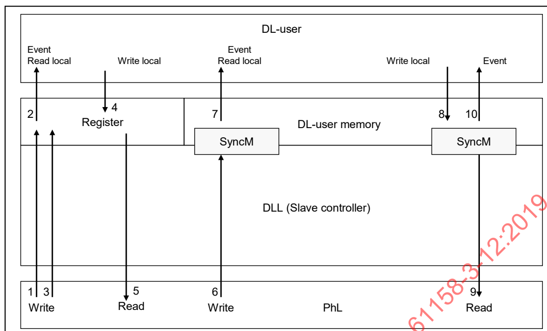
Figure 7 – Layering of communication
