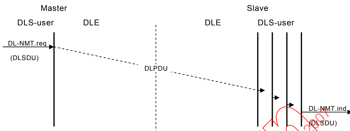
Figure 10 – Sequence diagram of a NMT-status transfer service
