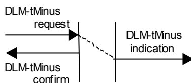
Figure 92 – Sequence of primitives for a DLM-tMinus change request
