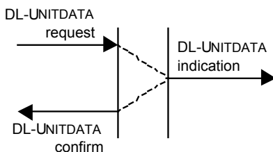
Figure 68 – Sequence of primitives for a successful remotely-acknowledged connectionless-mode unitdata transfer
