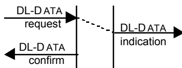
Figure 45 – Sequence of primitives for an ORDERED or UNORDERED peer-to-peer, or an UNORDERED subscriber-to-publisher queue-to-queue data transfer
