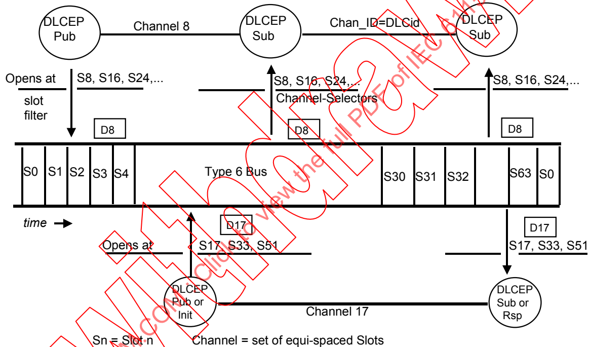
Figure 112 – EXAMPLE: TDMA bus operation using slots and channels.
