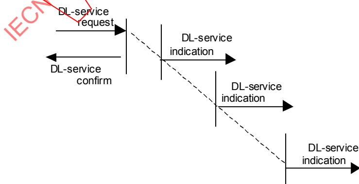
Figure 82 – DLS primitive time-sequence diagram
