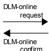
Figure 98 – Sequence of primitives for a DLM-online request
