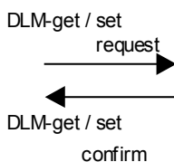
Figure 91 – Sequence of primitives for a DLM-get/set parameters request
