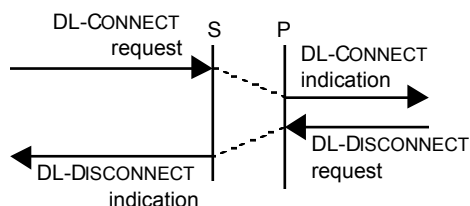
Figure 36 – Sequence of primitives in a publishing DLS-user rejection of a DLC/DLCEP establishment attempt
