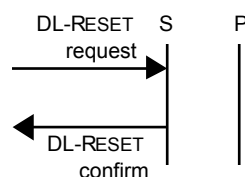
Figure 62 – Sequence of primitives in a simultaneous subscribing DLS-user and DLS-provider initiated Reset
