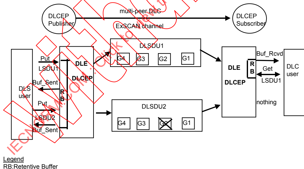
Figure 115 – The operation of the ExSCAN channel-class and its DLS-user interaction
