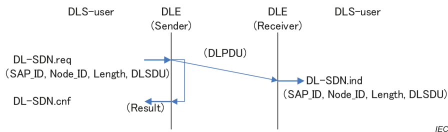
Figure 3 – Sequence of primitive for send data with no-acknowledge service
