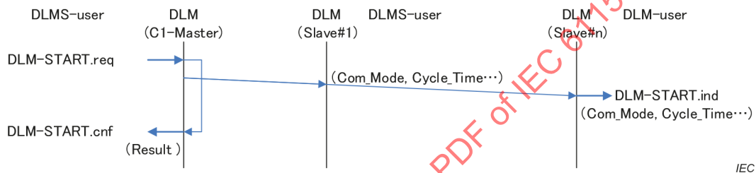
Figure 8 – Sequence of primitives for Start communication service
