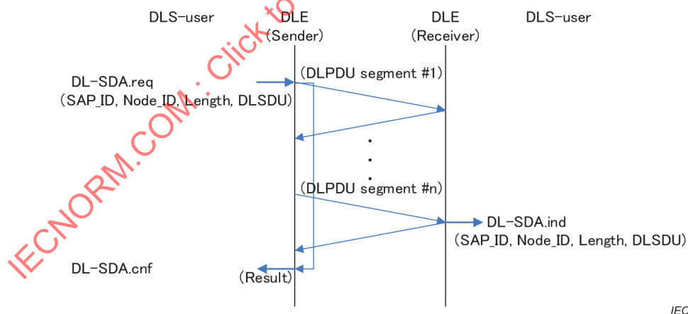
Figure 2 – Sequence of primitive for send data with acknowledge service
