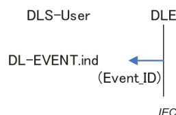
Figure 4 – Sequence of primitives for event service
