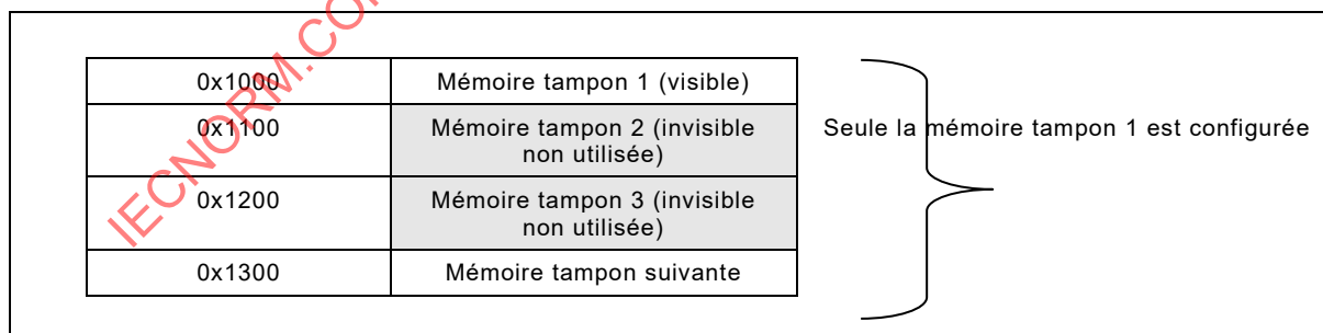
Figure 33 – Attribution de mémoire tampon SyncM
