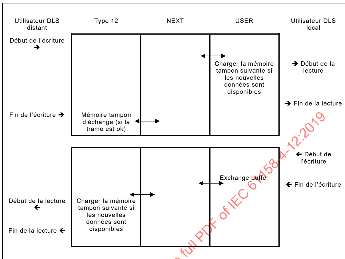
Figure 34 – Interaction de mémoire tampon SyncM
