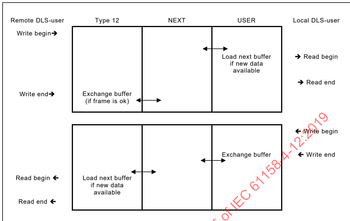
Figure 34 – SyncM buffer interaction
