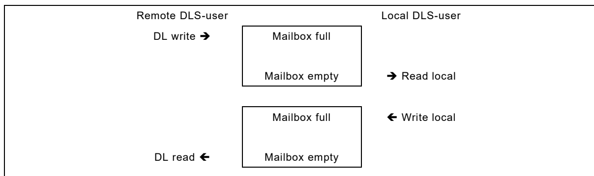
Figure 32 – SyncM mailbox interaction
