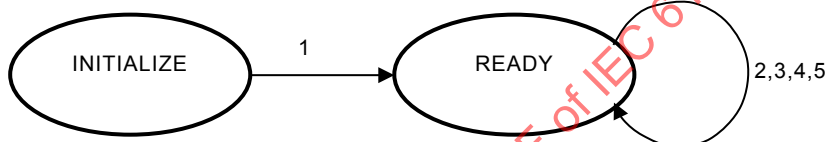
Figure 15 – State transition diagram of ITC
