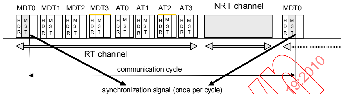
Figure 13 – Synchronization timing
