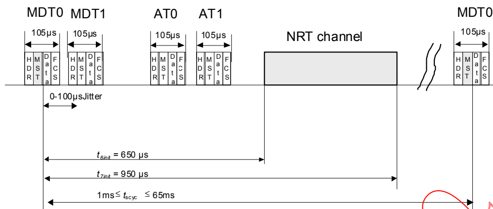
Figure 11 – Timing diagram of CP1 and CP2 with 2 MDT/AT
