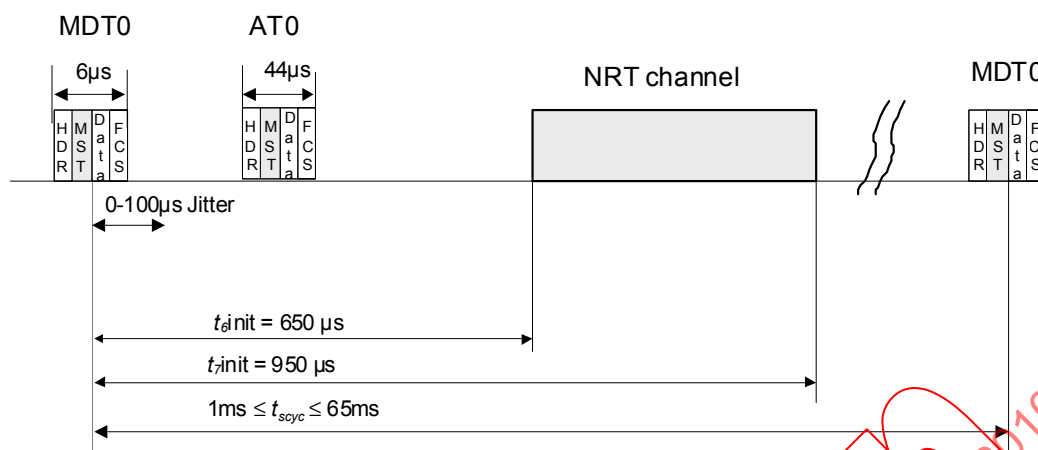
Figure 10 – Timing diagram of CP0
