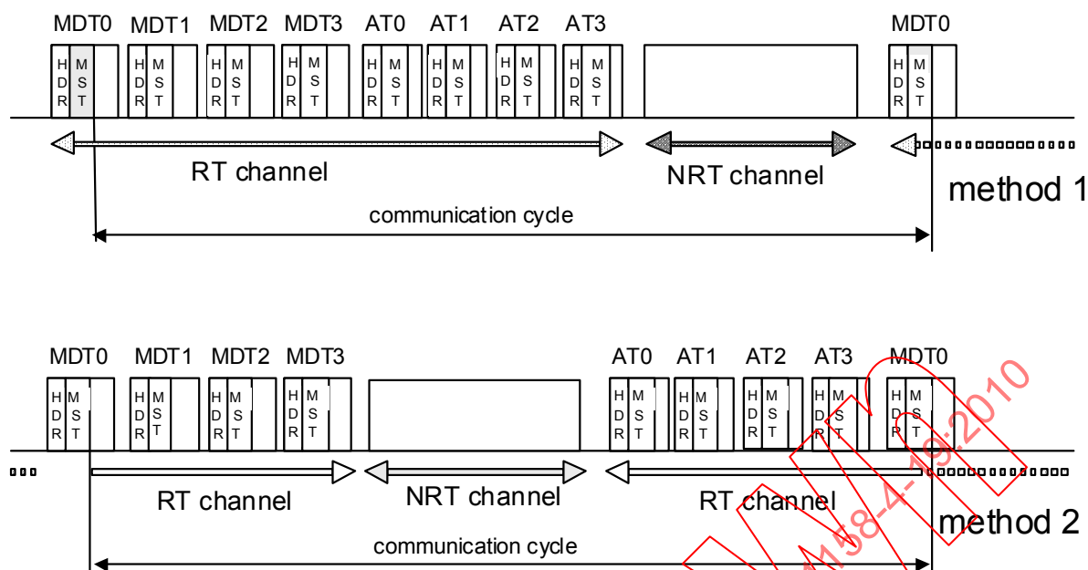
Figure 7 – Telegram sequence
