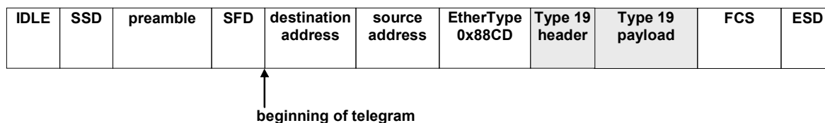
Figure 8 – Beginning of telegram
