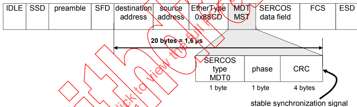
Figure 14 – Synchronization signal generation
