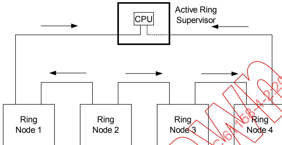
Figure 25 – Normal operation of a DLR network
