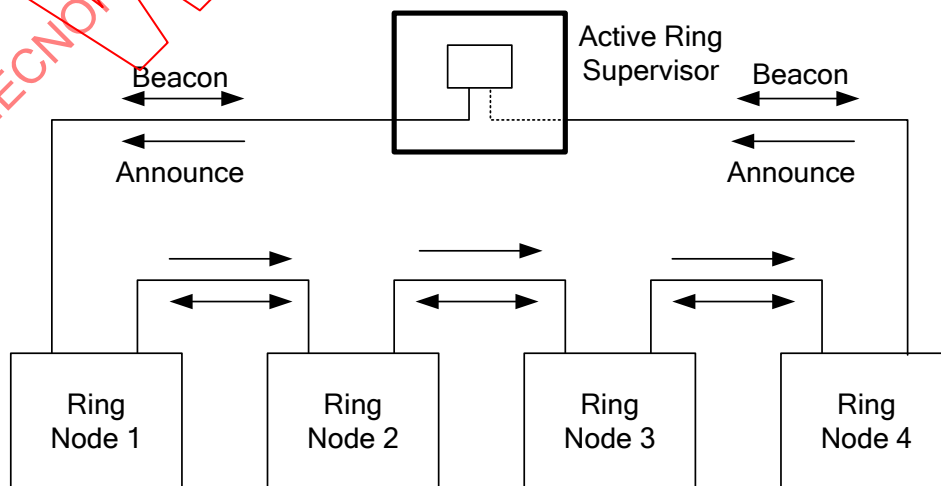
Figure 26 – Beacon and Announce frames
