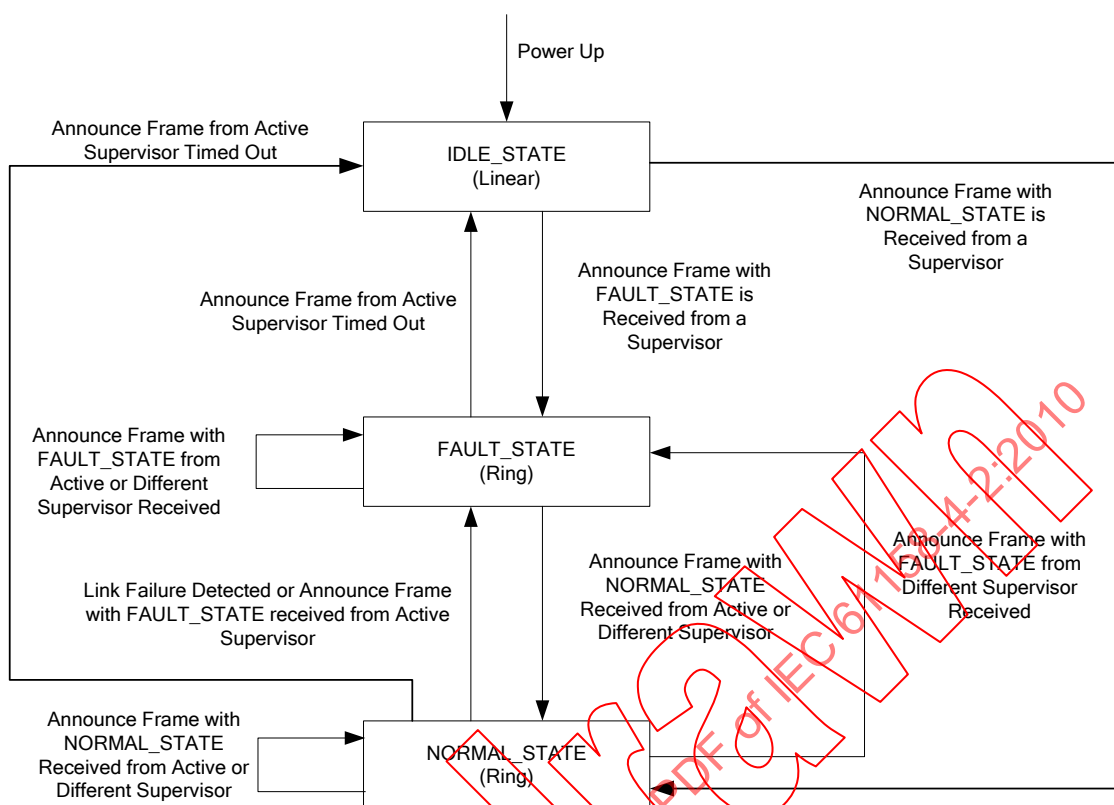
Figure 33 – State transition diagram for Announce frame based non-supervisor ring node
