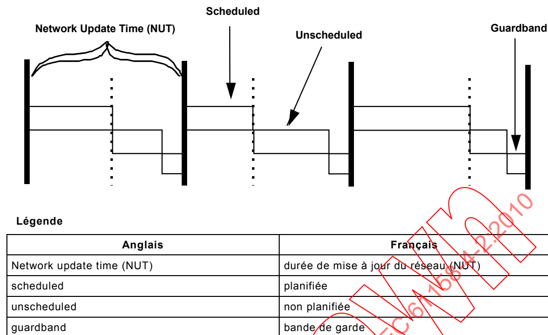
Figure 7 – Structure de la NUT
