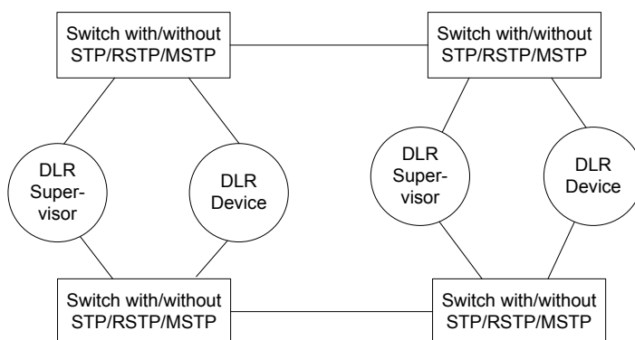
Figure 30 – Unsupported topology – example 1
