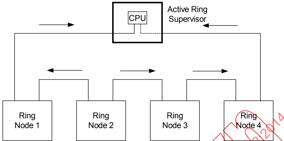
Figure 28 – Normal operation of a DLR network
