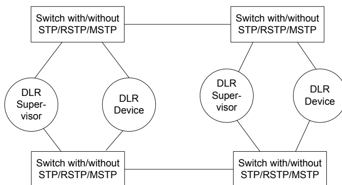
Figure 33 – Unsupported topology – example 1
