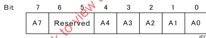
Figure 17 – Cyclic transmission frame address
