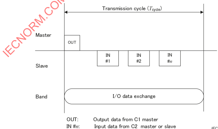
Figure 6 – Timing chart of no time slot type cyclic communication (Master send common address)
