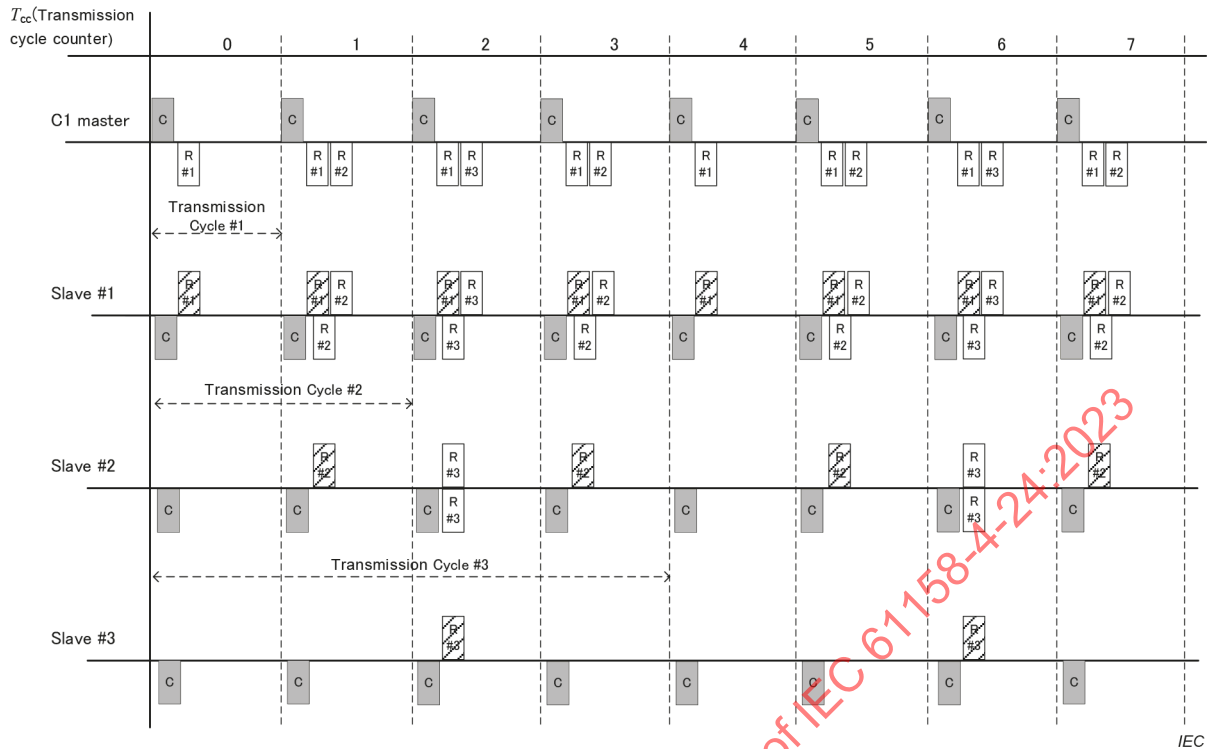
Figure 8 – Timing chart for multiple transmission cycle setting
