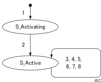
Figure 28 – The state diagram of the C2 master for no time slot type
