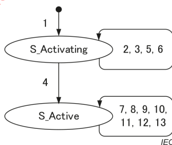
Figure 26 – The state diagram of slave for configurable time slot
