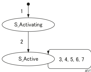
Figure 29 – The state diagram of the Slave for no time slot type
