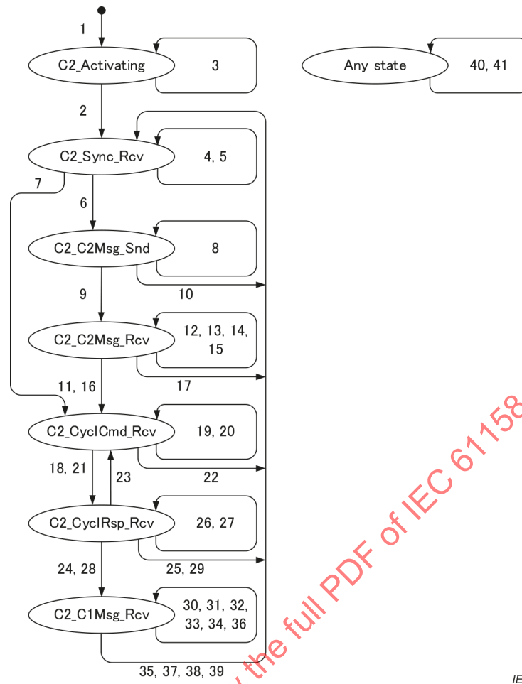
Figure 22 – The state diagram of the C2 master for fixed-width time slot
