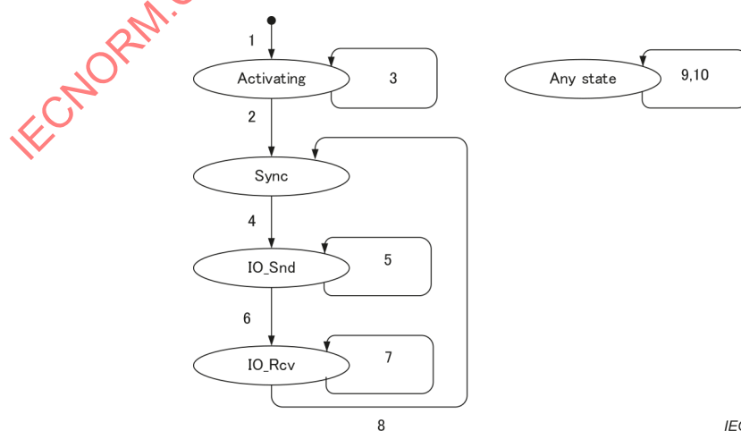
Figure 27 – The state diagram of the C1 master for no time slot type
