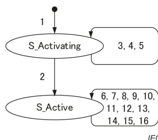
Figure 23 – The state diagram of the slave for fixed-width time slot
