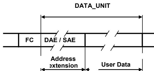
Figure 22 – Data field
