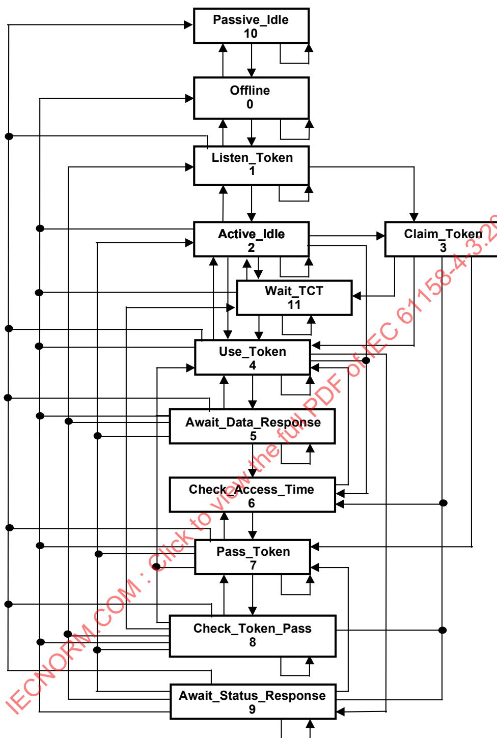
Figure 38 – DL-state-diagram
