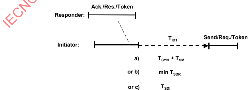
Figure 4 – Idle time T_{ID1}
