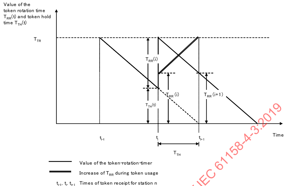
Figure C.1 – Derivation of the token holding time ( T_{TH} )
