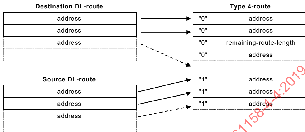
Figure 18 – Complex and IP Type 4-route generation
