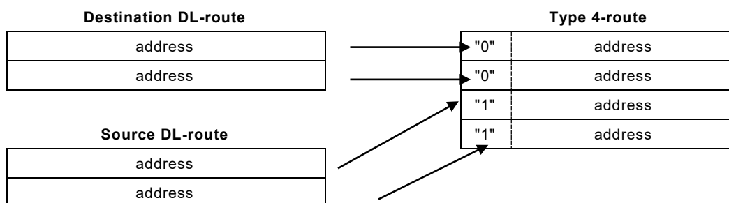
Figure 17 – Extended Type 4-route generation
