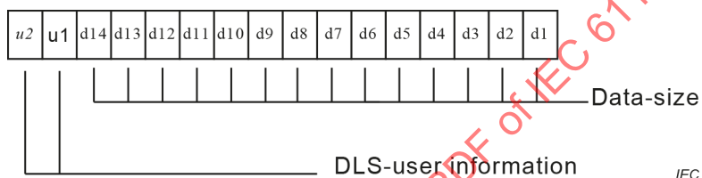
Figure 15 – Data field format, two octets
