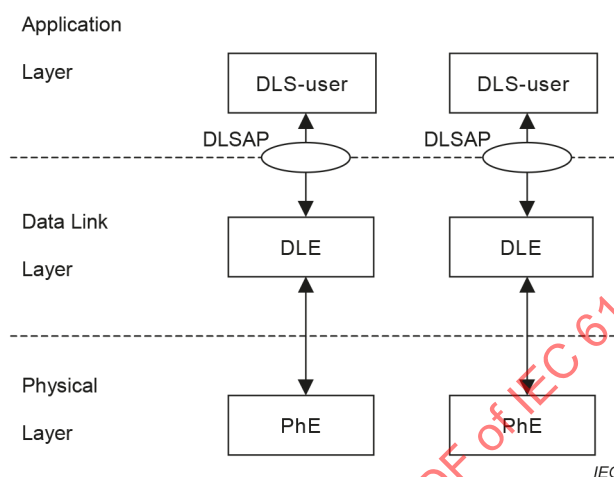
Figure 1 – Relationship of PhE, DLE and DLS-user
