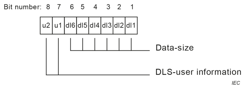
Figure 14 – Data-field-format, one octet
