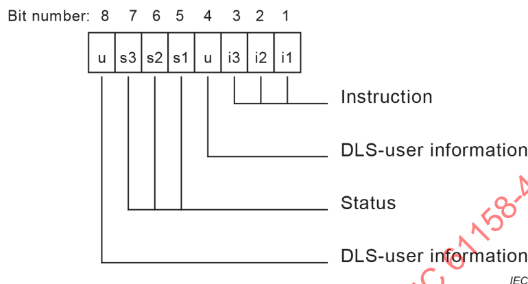
Figure 13 – Control-status format
