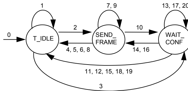
Figure 39 – Machine de protocole TRANSMIT
