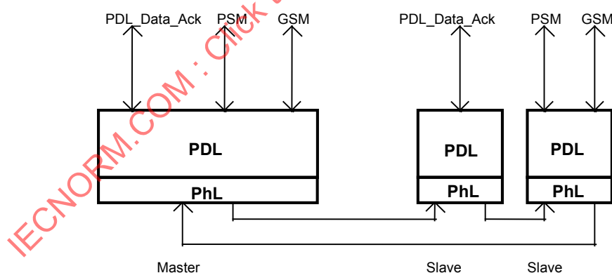
Figure 8 – Overview of the PDL services
