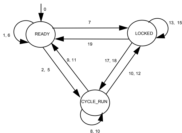
Figure 48 – Machine de protocole BLL-BAC
