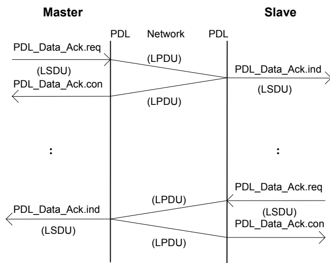
Figure 9 – PDL_Data_Ack service between master and only one slave
