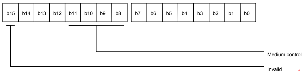
Figure 83 – Structure of the control code
