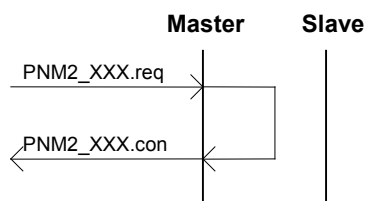
Figure 77 – Reset, Set Value, Get Value and Get Active Configuration services
