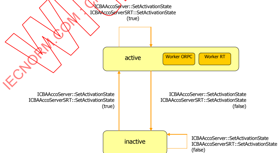
Figure 42 – State machine ProviderConnection
