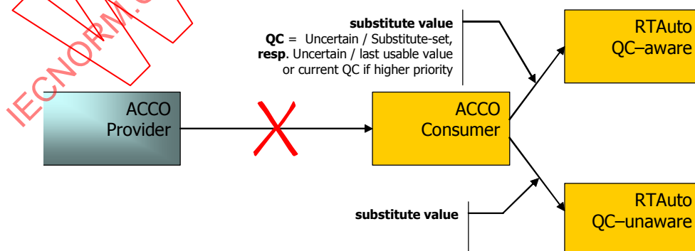
Figure 23 – Quality code with communication fault
