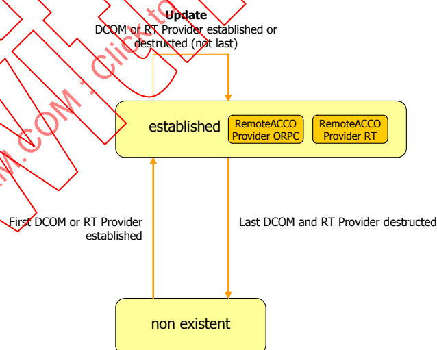
Figure 38 – State machine RemoteACCOProvider
