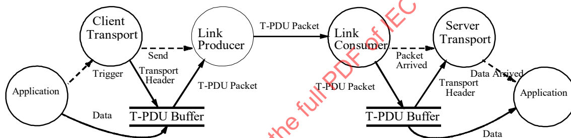
Figure 23 – Data flow diagram for a link producer
