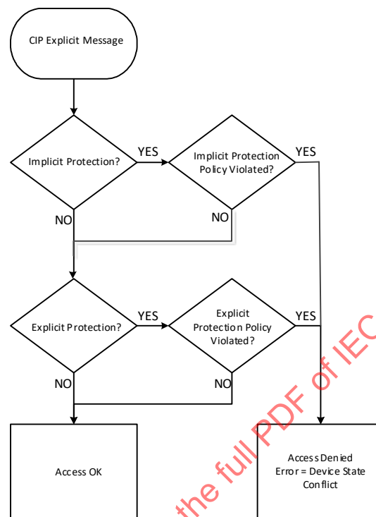
Figure 4 – Explicit and Implicit Setting interaction
