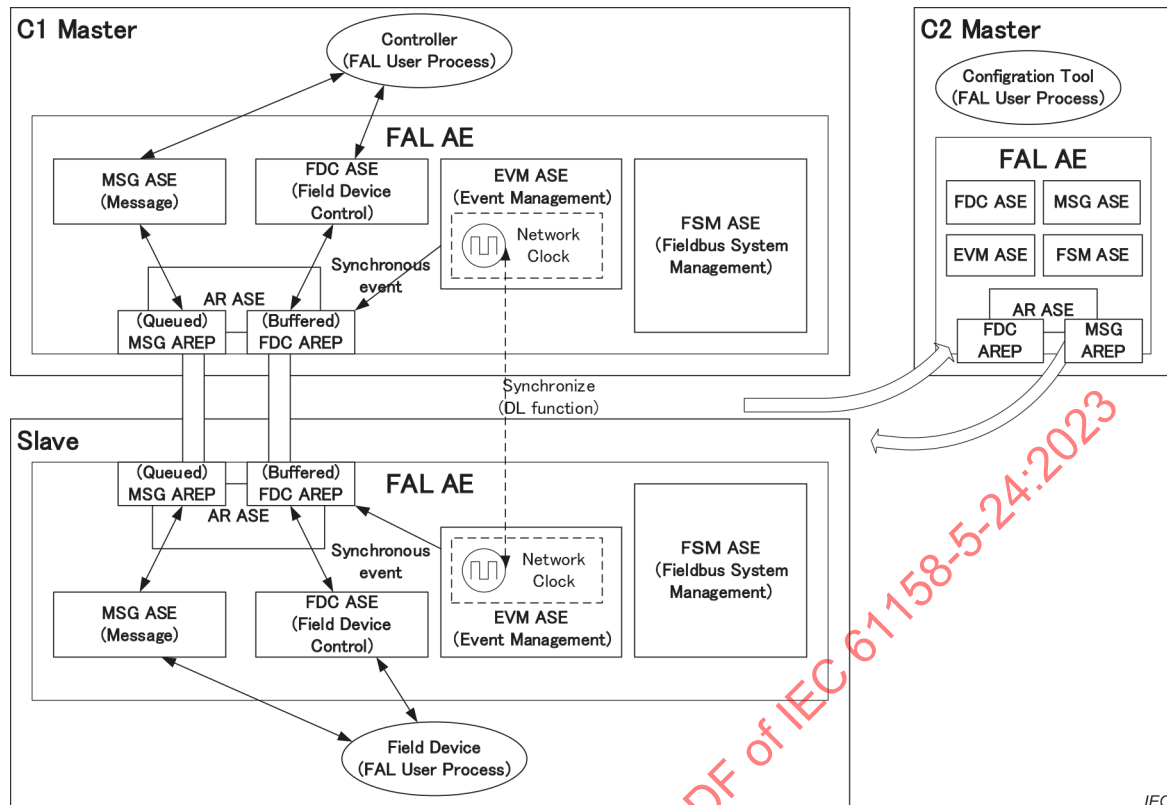
Figure 1 – FAL ASE model of Type 24
