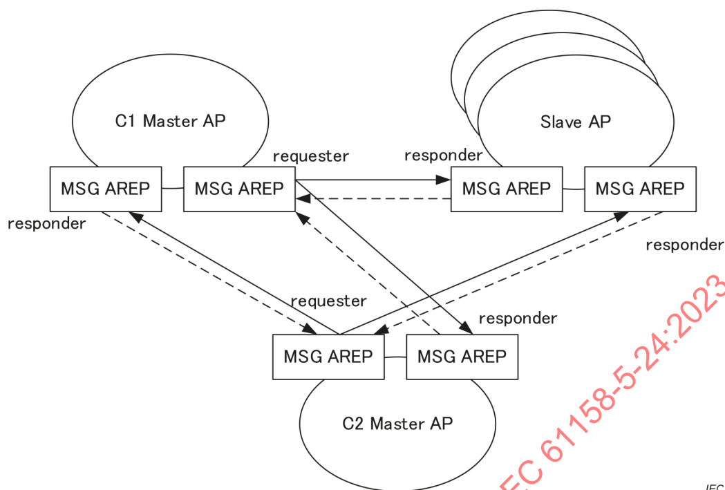
Figure 4 – MSG ARs between each APs
