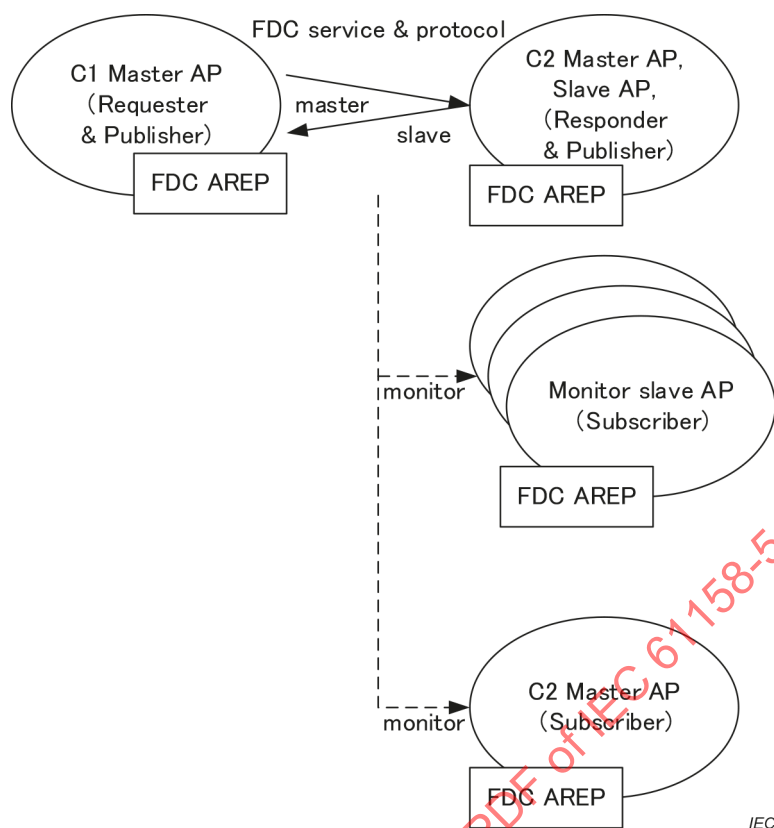
Figure 2 – AR model for field device control service
