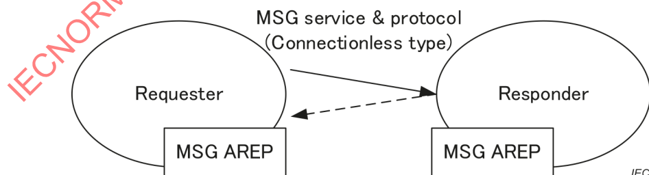
Figure 3 – AR model for message service
