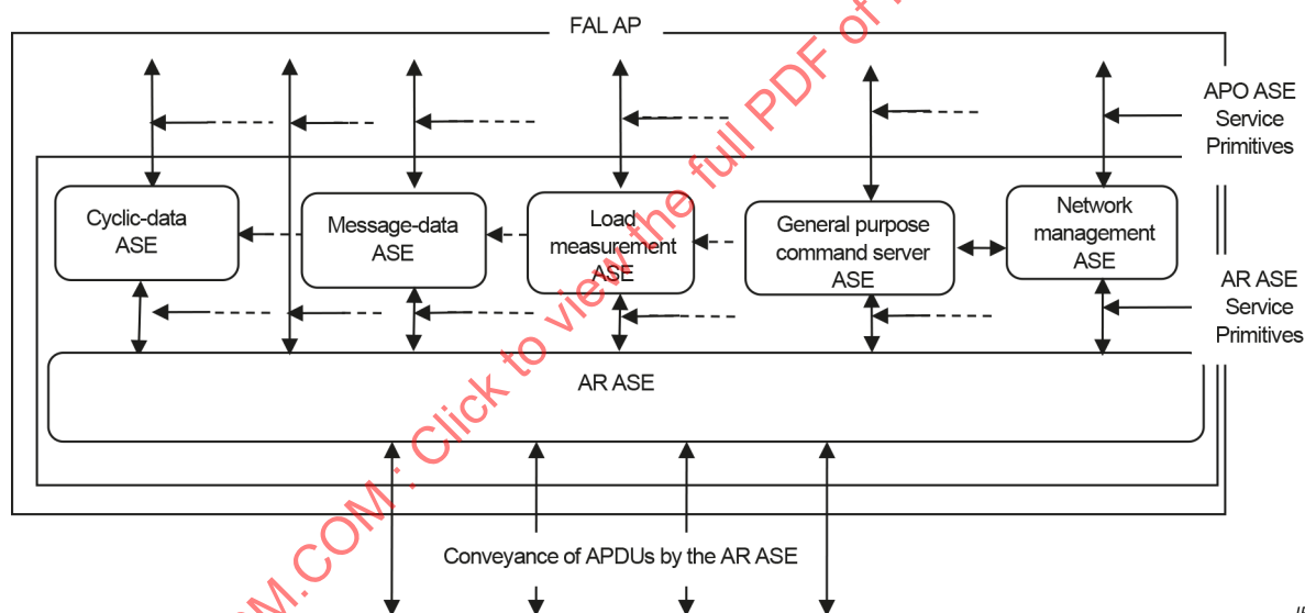
Figure 9 – The structure of ASEs for Type 26 FAL
