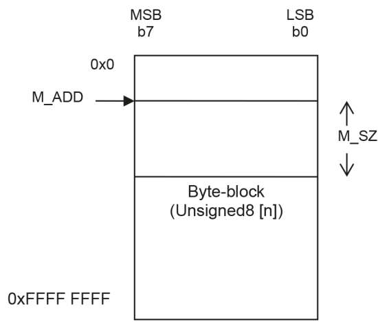
Figure 10 – Virtual-address-space for Byte block
