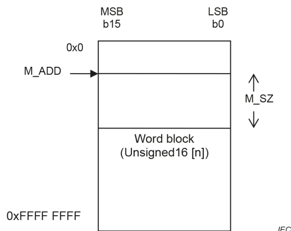
Figure 11 – Virtual-address-space for Word block
