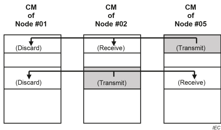
Figure 7 – Node #01 without the CM
