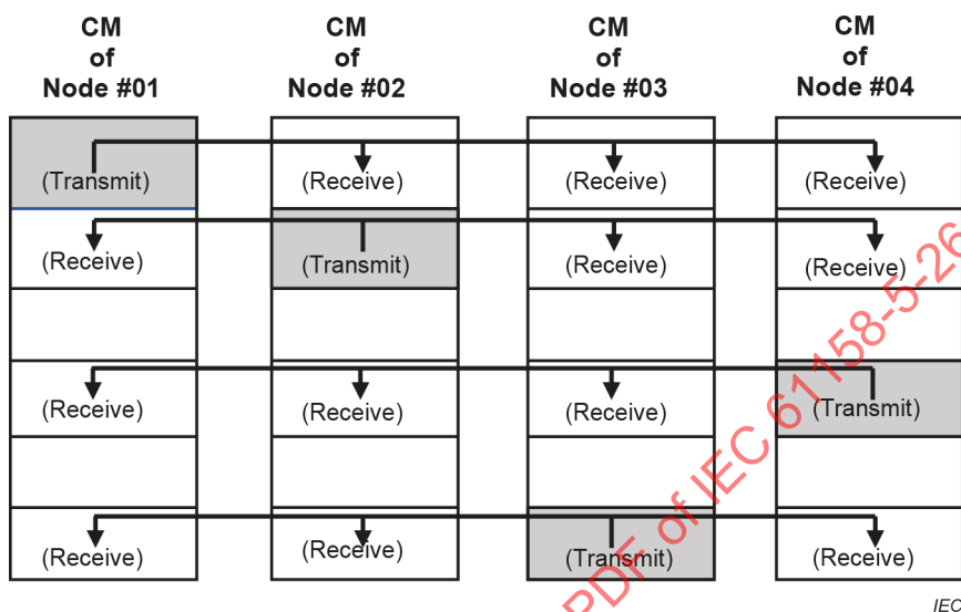
Figure 5 – Data sharing with the CM
