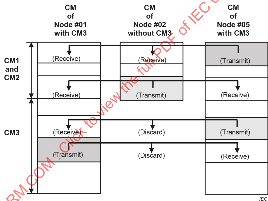
Figure 8 – Data sharing among nodes with and without CM3
