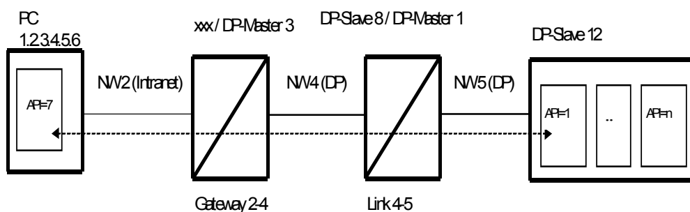
Figure 40 – Second example with inter-network addressing
