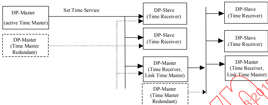
Figure 28 – System architecture
