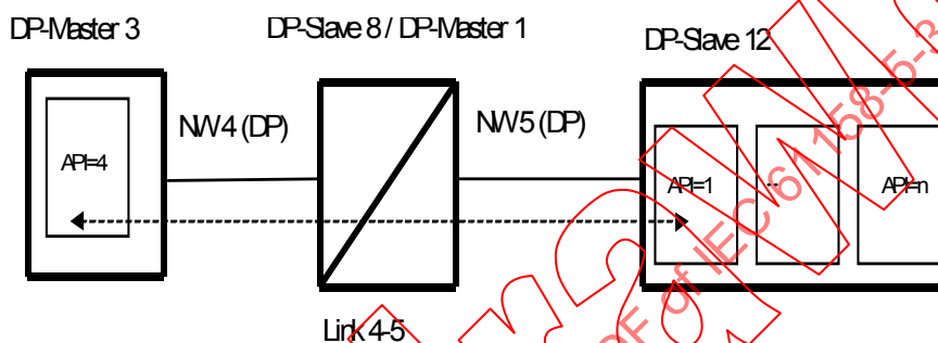
Figure 39 – First example with inter-network addressing
