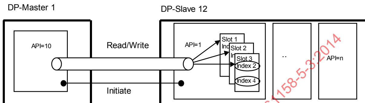
Figure 38 – Example without inter-network addressing
