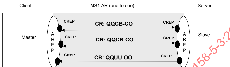
Figure 35 – MS1 application relationship
