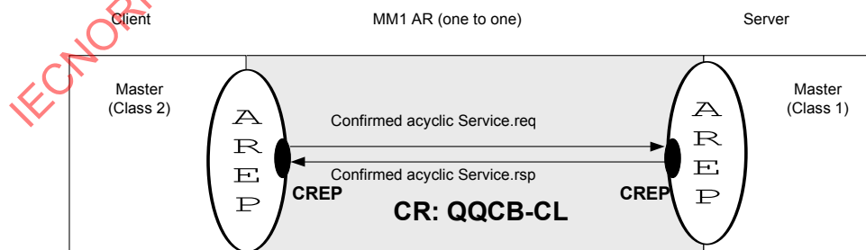
Figure 42 – MM1 application relationship
