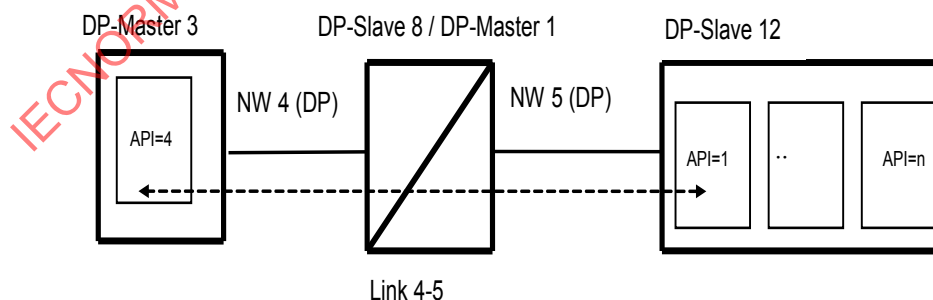
Figure 39 – First example with inter-network addressing
