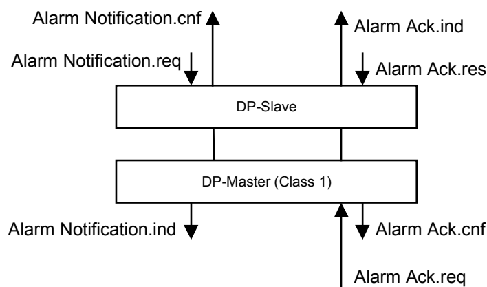
Figure 24 – Treatment of an alarm in the DP system
