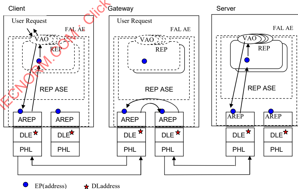
Figure 14 – Summary of the FAL architecture
