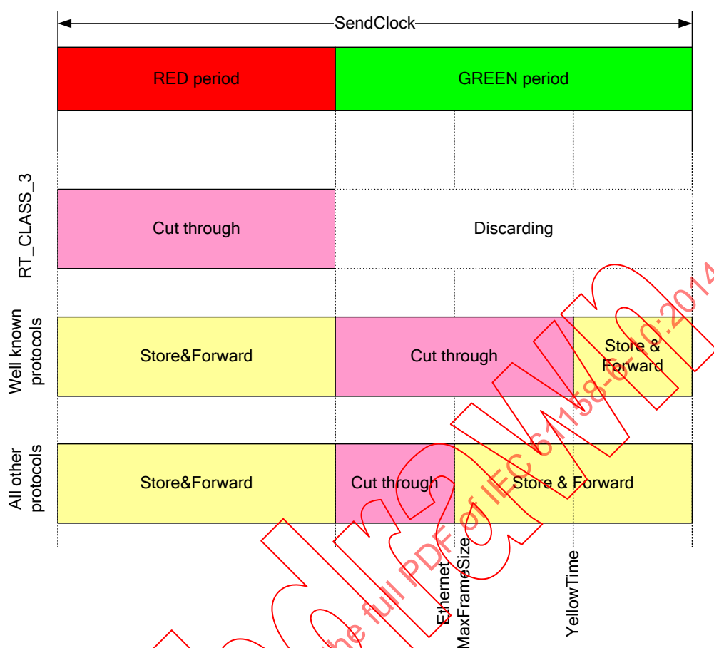
Figure 85 – Calculation principle for the minimum YellowTime
