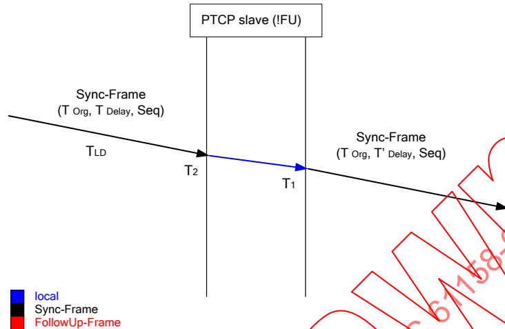
Figure 36 – !FU Sync Slave Forwarding Sync-Frame
