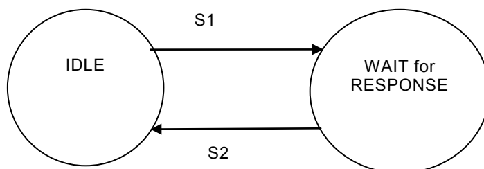
Figure 11 – State transition diagram of the server ARPM
