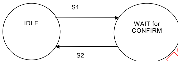
Figure 10 – State transition diagram of the client ARPM
