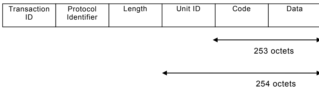
Figure 14 – TCP/IP PDU format
