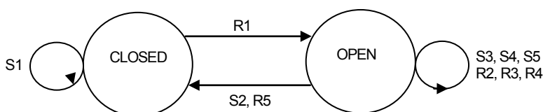
Figure 17 – State transition diagram of the MSU-ARPM
