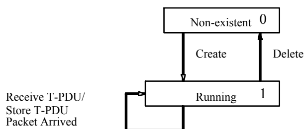
Figure 59 – State transition diagram for a link consumer
