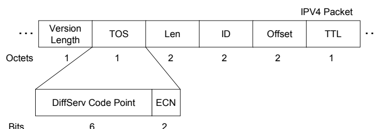
Figure 60 – DS field in the IP header
