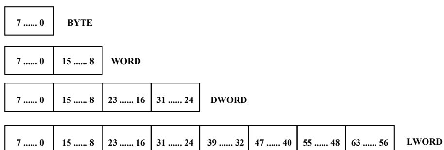
Figure 15 – FixedLengthBitString compact encoding bit placement rules
