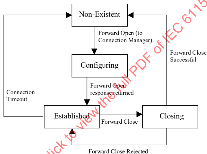
Figure 30 – Bridged Connection object state transition diagram
