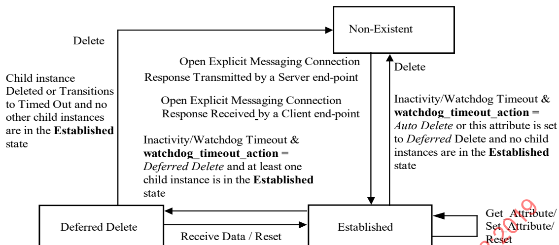
Figure 31 – Explicit Messaging Connection object state transition diagram
