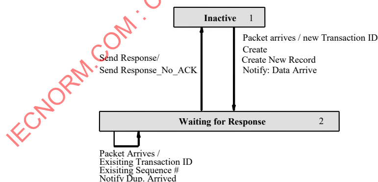
Figure 34 – State transition diagram of low-end UCMM server
