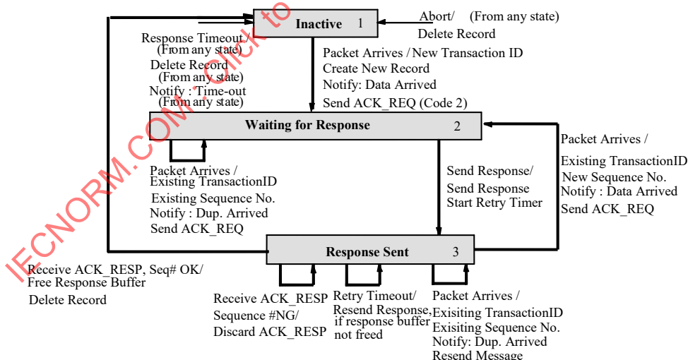
Figure 33 – State transition diagram of high-end UCMM server
