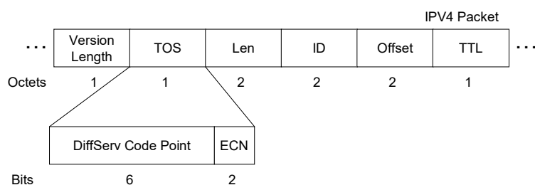
Figure 59 – DS field in the IP header
