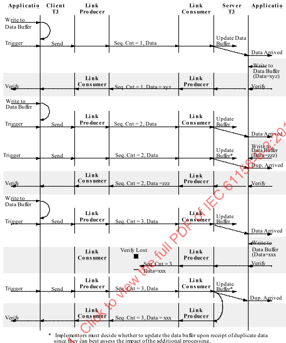
Figure 53 – Sequence diagram of data transfer using client transport class 3 and server transport class 3 with returned data
