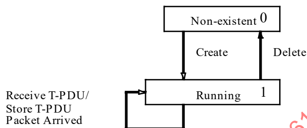
Figure 58 – State transition diagram for a link consumer
