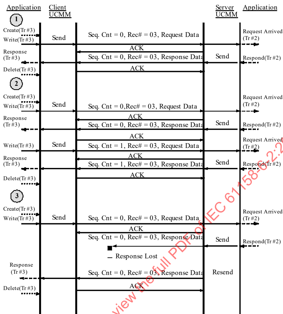
Figure 35 – Sequence diagram for a UCMM with one outstanding message
