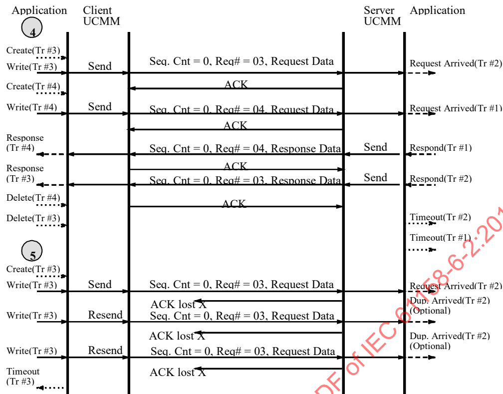
Figure 36 – Sequence diagram for a UCMM with multiple outstanding messages
