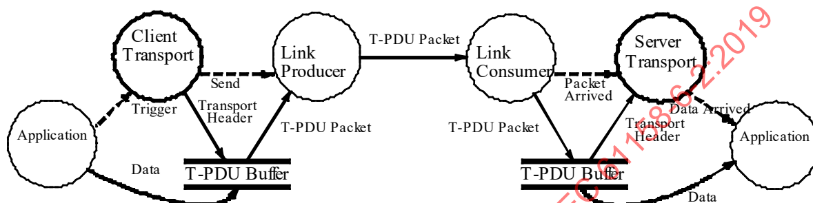
Figure 37 – TPDU buffer
