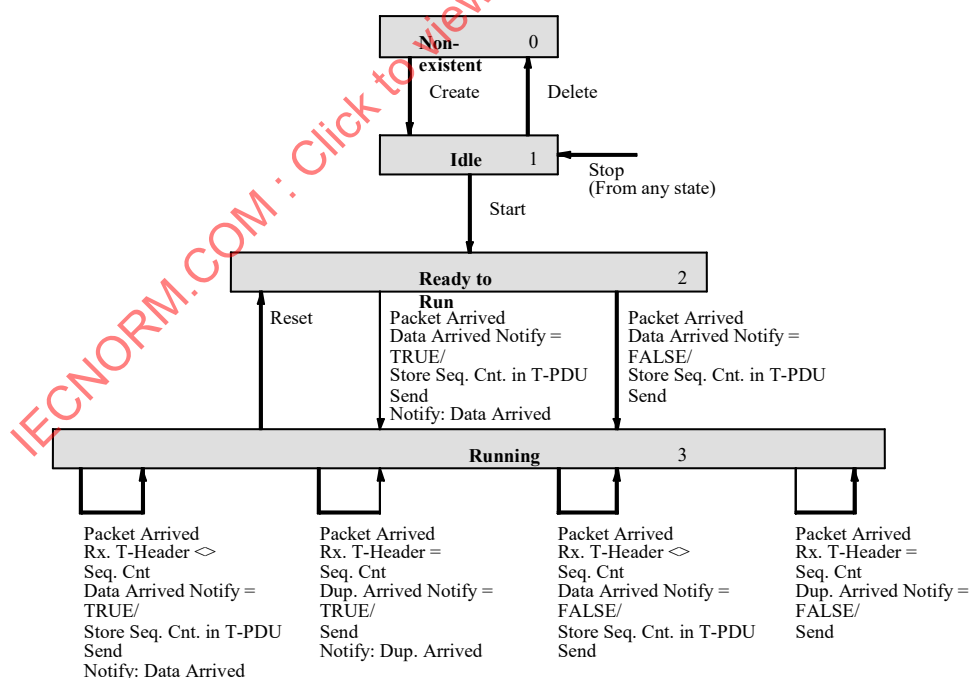
Figure 50 – Class 2 server STD
