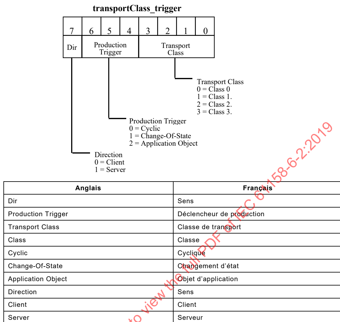
Figure 7 – Attribut Transport Class Trigger
