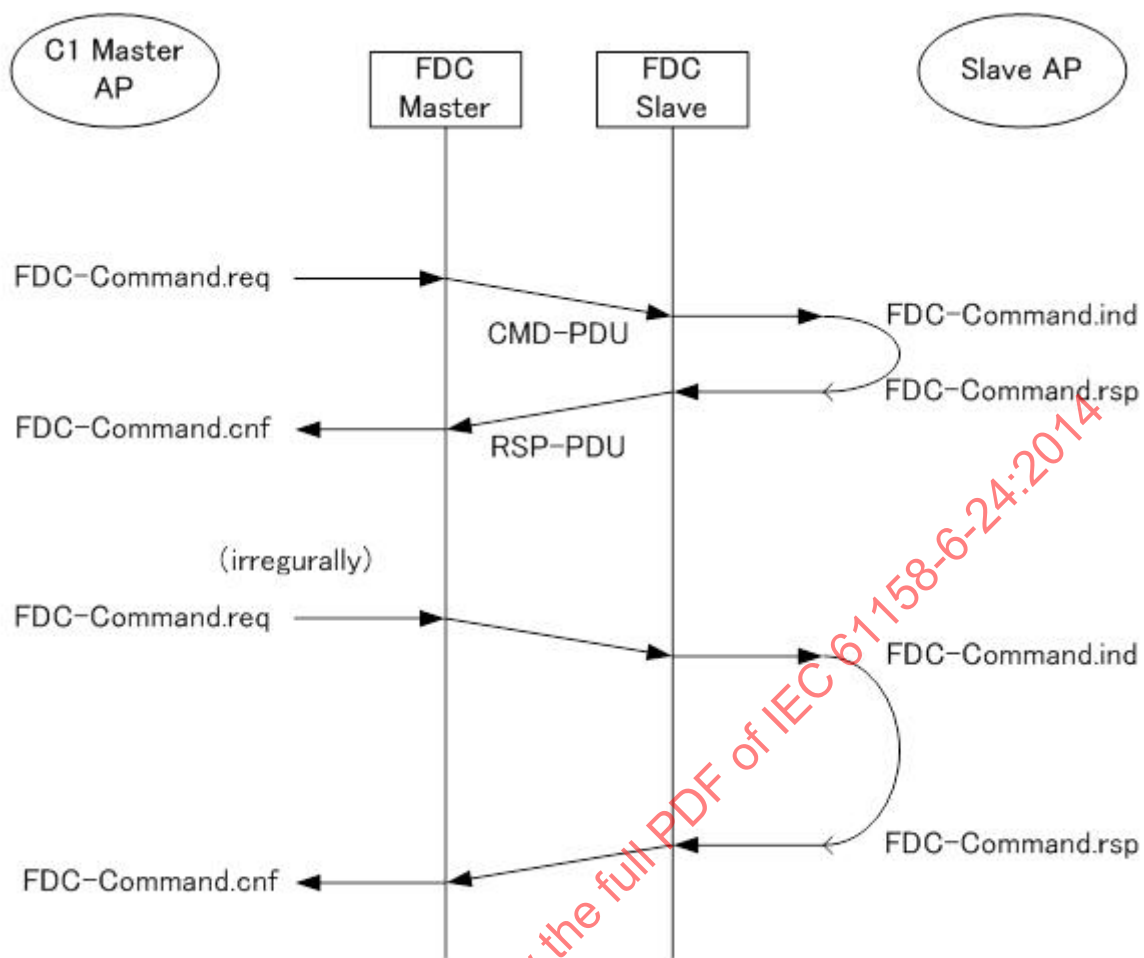
Figure 17 – Event-driven communication
