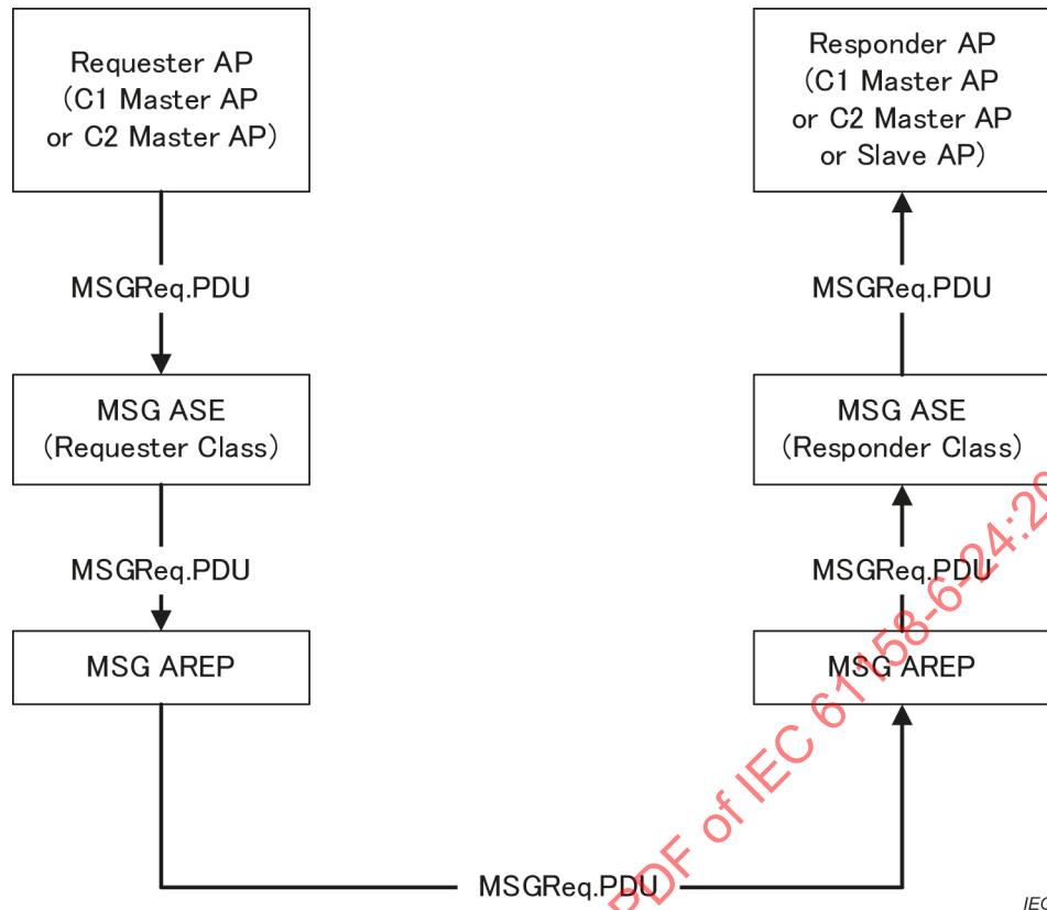
Figure 22 – PDU transmission flow for one-way message
