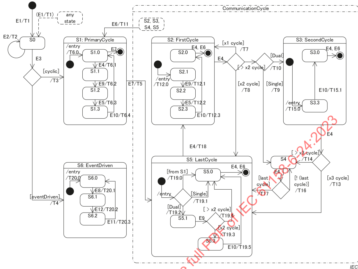
Figure 29 – Statechart diagram of ARPM-FDCM
