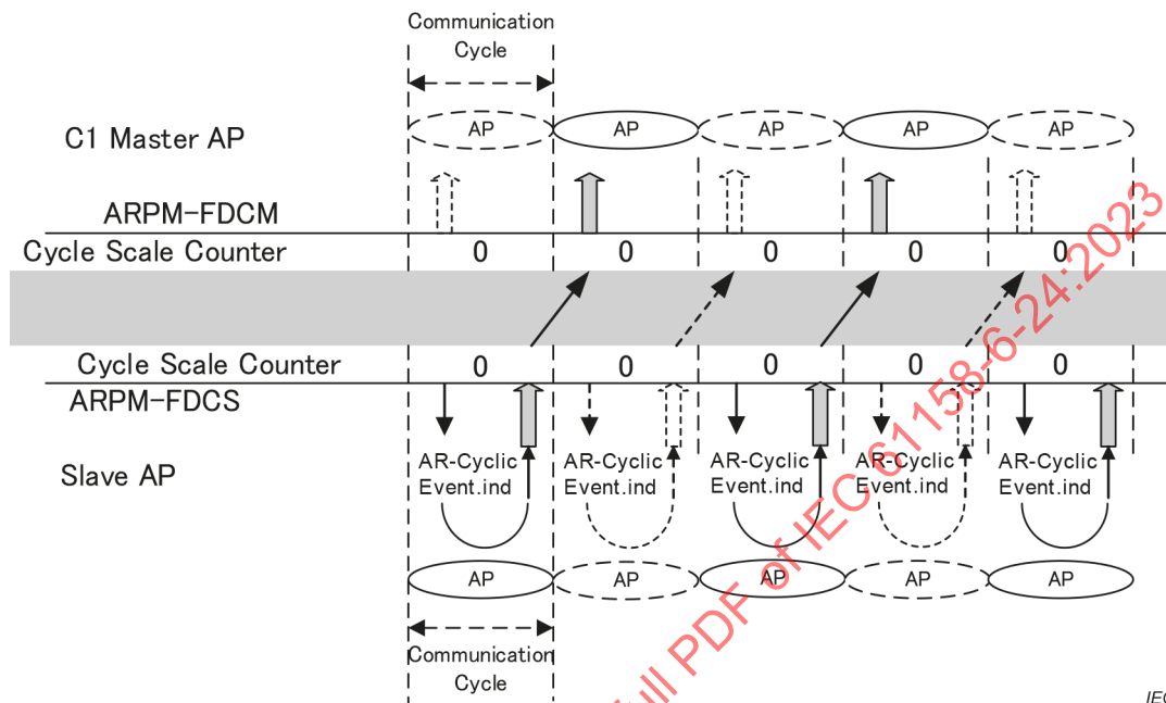
Figure 27 – Example of Synchronous command communication
