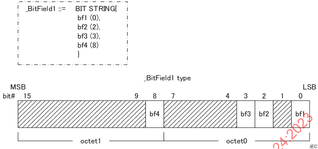
Figure 7 – Bit field definition example with named bits
