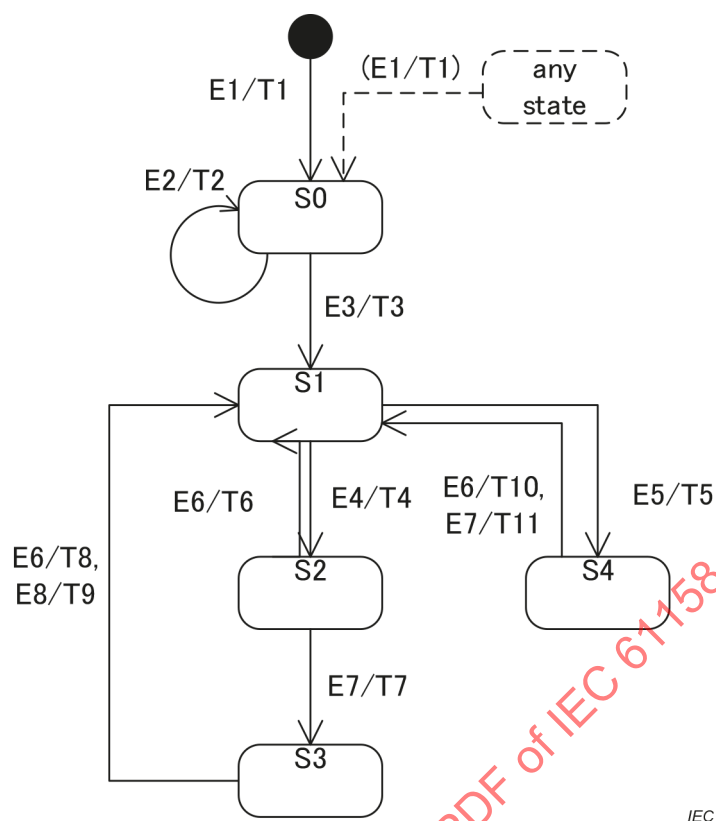
Figure 23 – Statechart diagram of MSGPM-RQ
