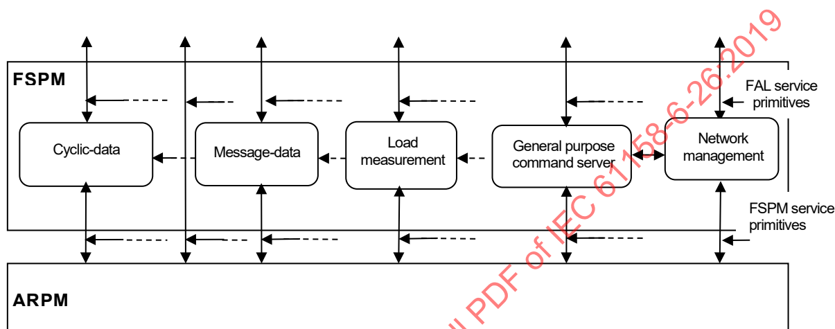
Figure 53 – Overall structure of FSPM
