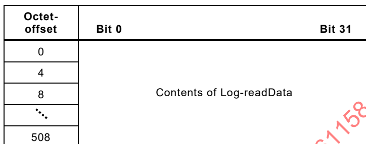
Figure 35 – Structure of Log-readData with M_RLT = 0
