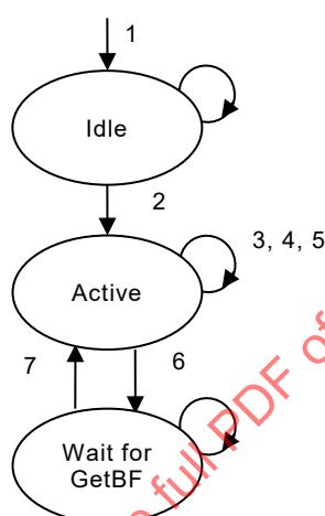
Figure 54 – State transition diagram of Cyclic-data protocol machine
