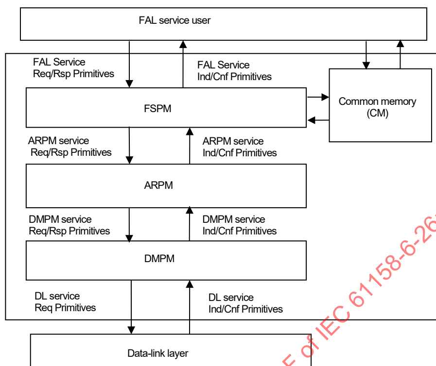
Figure 52 – Relationship between FAL protocol machines
