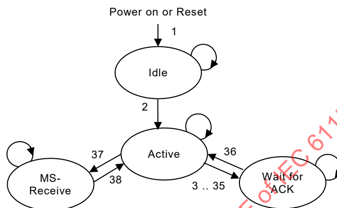
Figure 55 – State transition diagram of Message-data protocol machine
