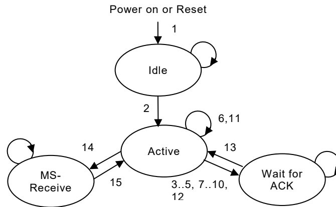
Figure 56 – State transition diagram of Load measurement protocol machine
